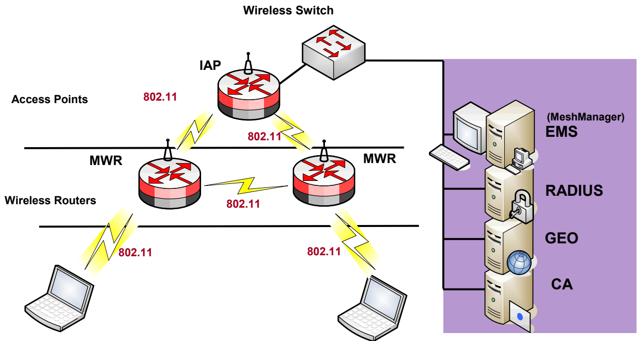
Figure 1-2 MWR and IAP Devices in Context of a MOTOMESH Network
