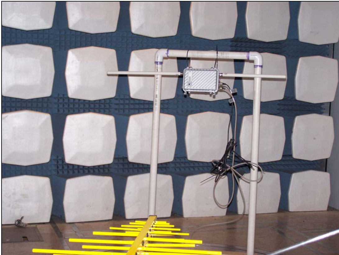
Photograph 2. Radiated Emissions
