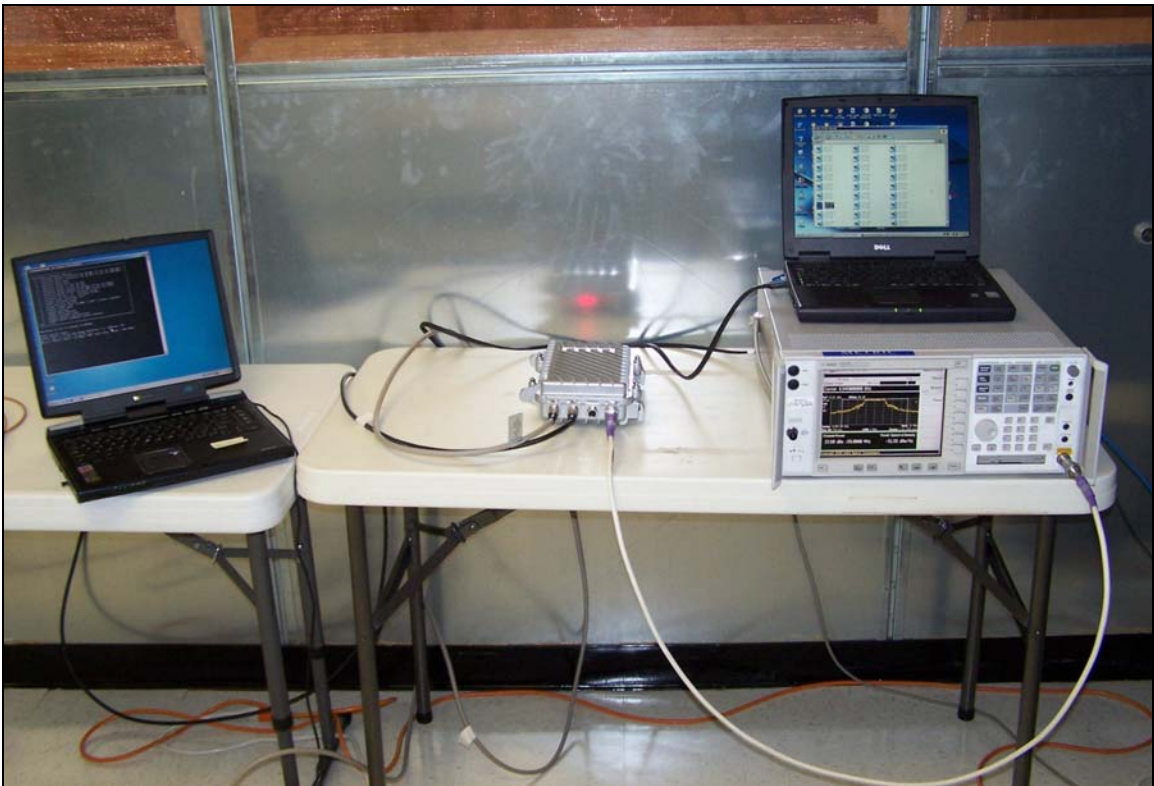
Photograph 4. Emissions Bandwidth
