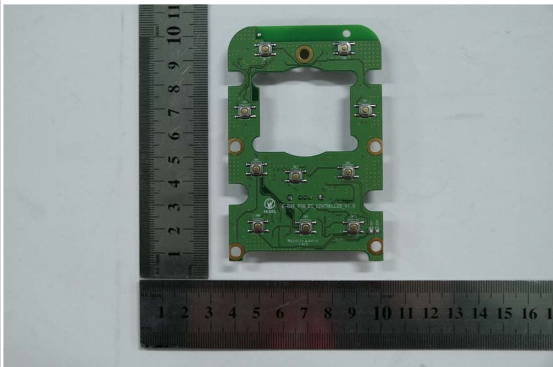
View of Main PCB(Bottom)
