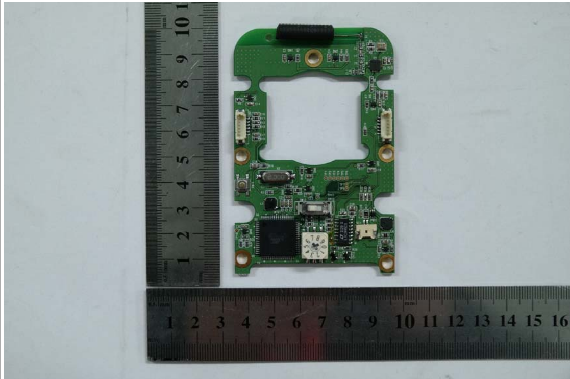
View of Main PCB(Top)
