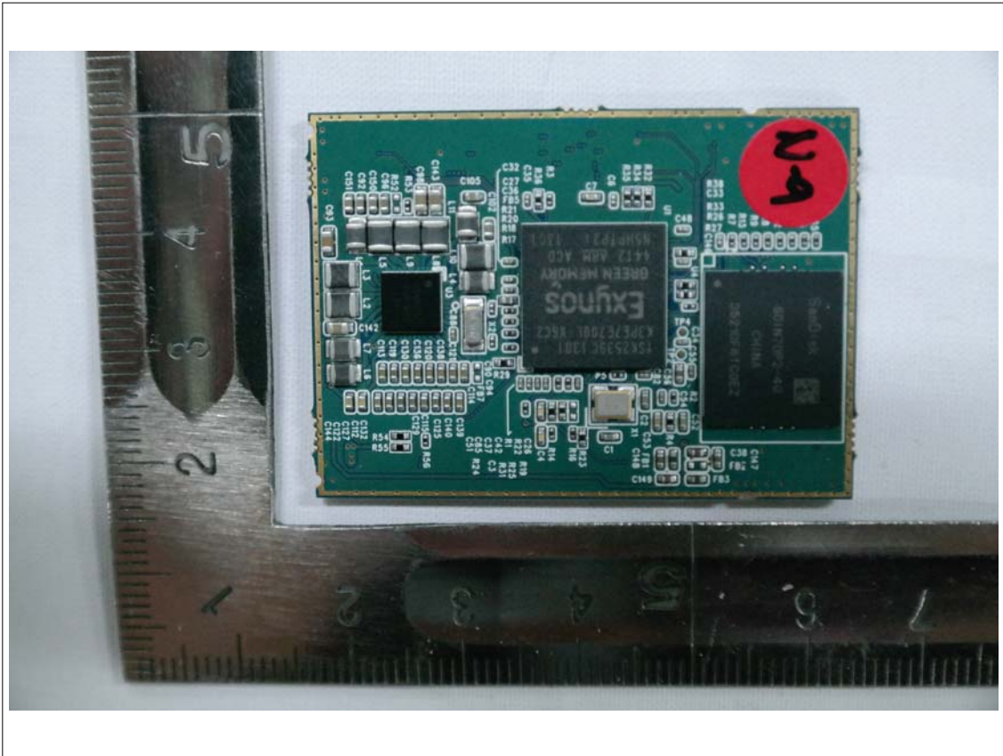
View of CPU PCB(Top)
