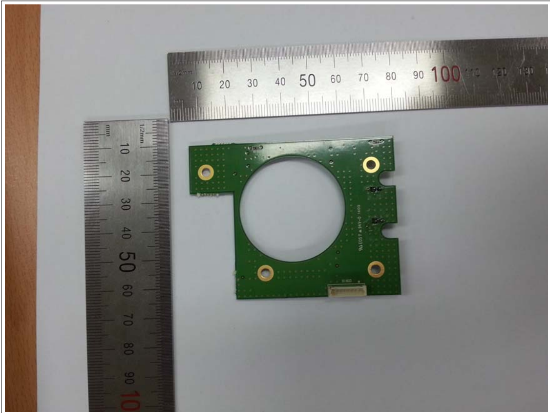
View of Sub PCB 7(Bottom)
