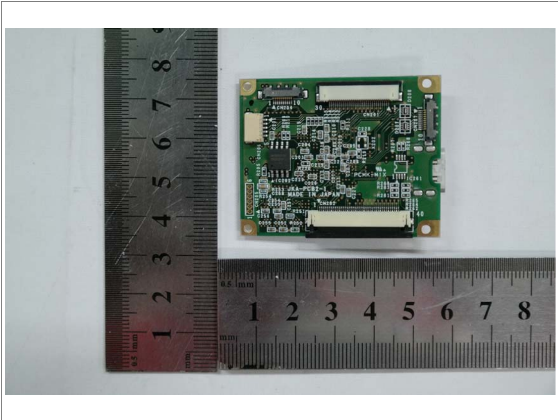
View of Sub PCB 6(Top)
