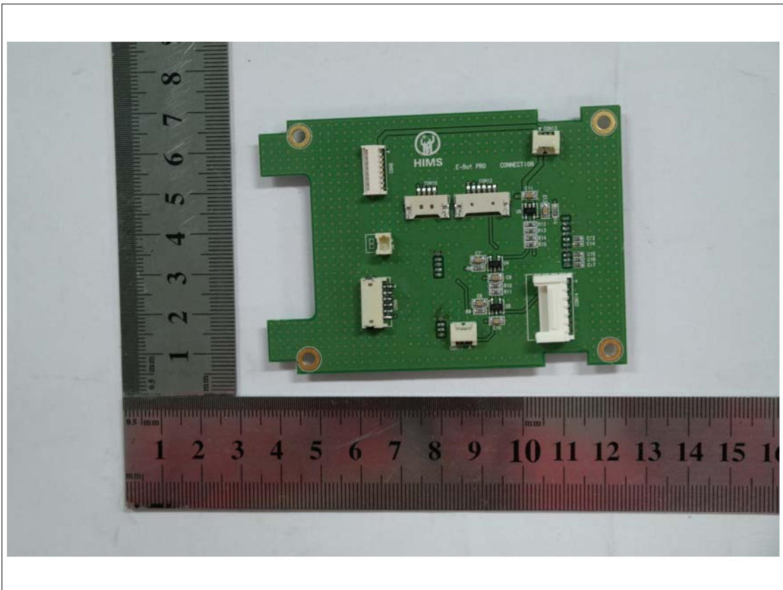
View of Sub PCB 4(Bottom)
