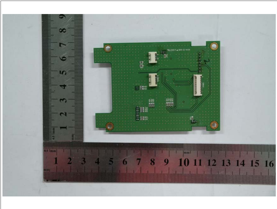
View of Sub PCB 4(Top)
