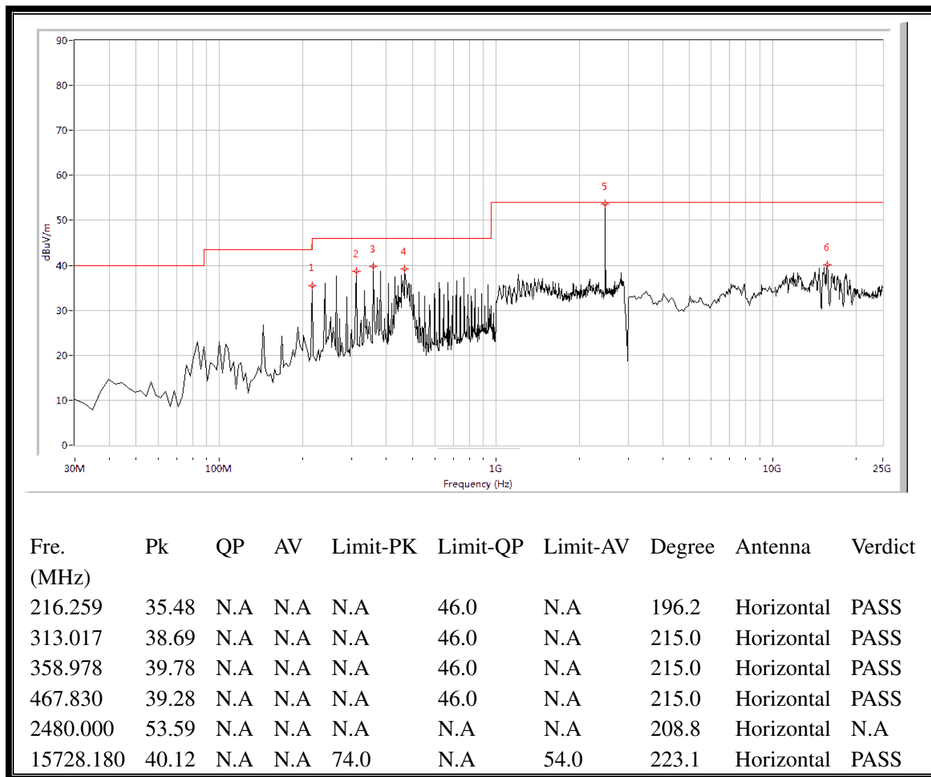
(Plot C.2: Antenna Horizontal, 30MHz to 25GHz)
