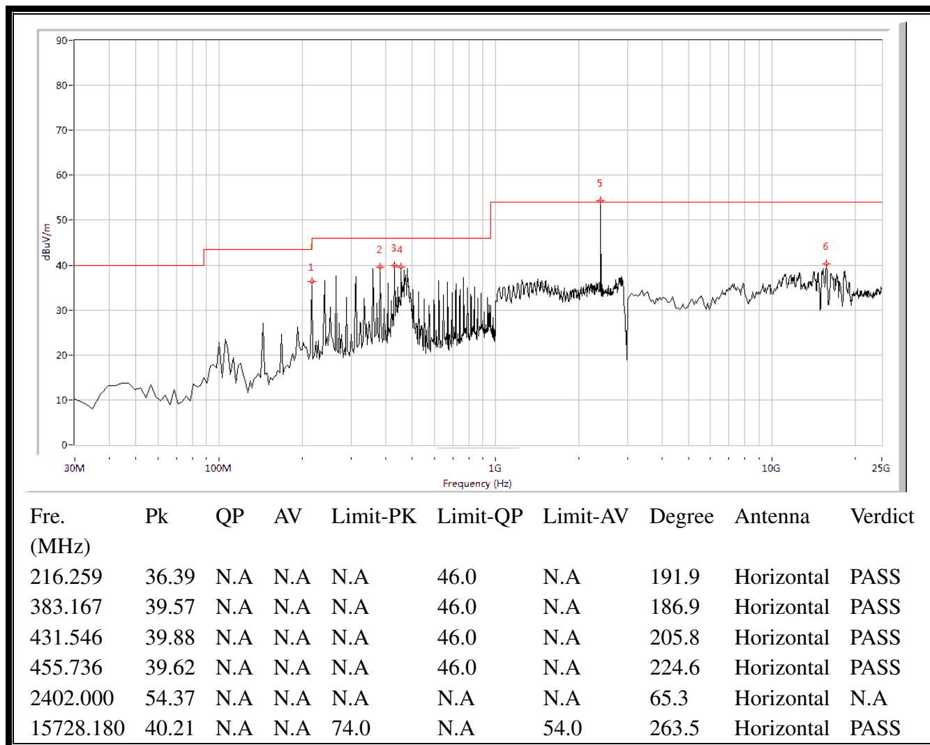
(Plot A.2: Antenna Horizontal, 30MHz to 25GHz)
