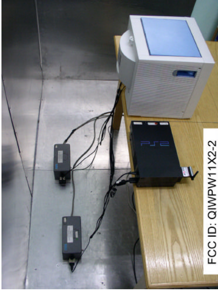
Side View
