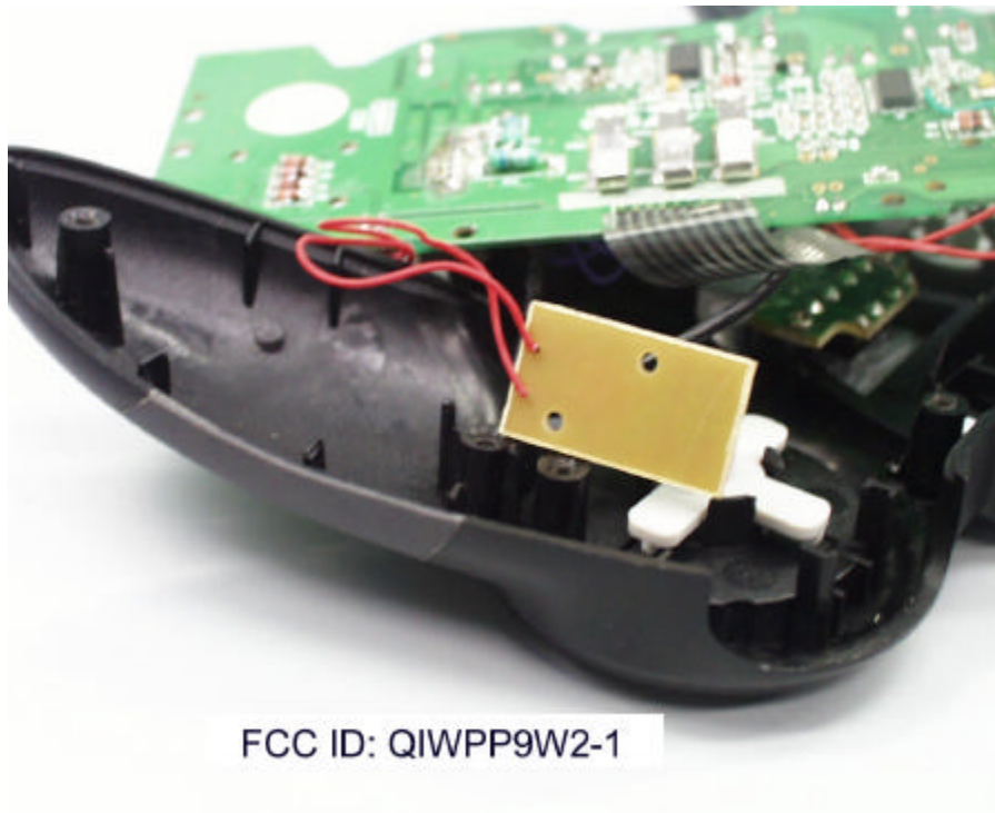
Switch PCB Photo 3
