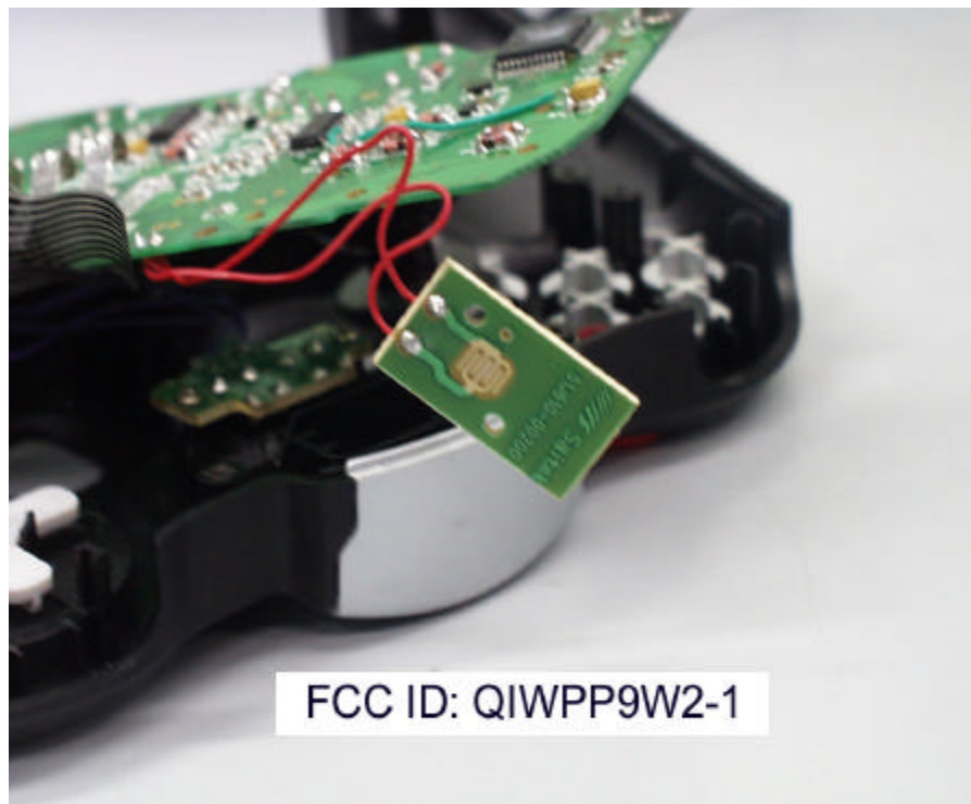
Switch PCB Photo 1
