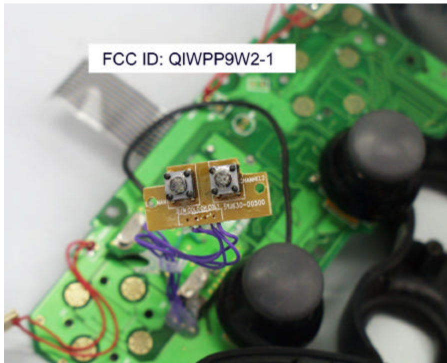
Switch PCB Photo 5
