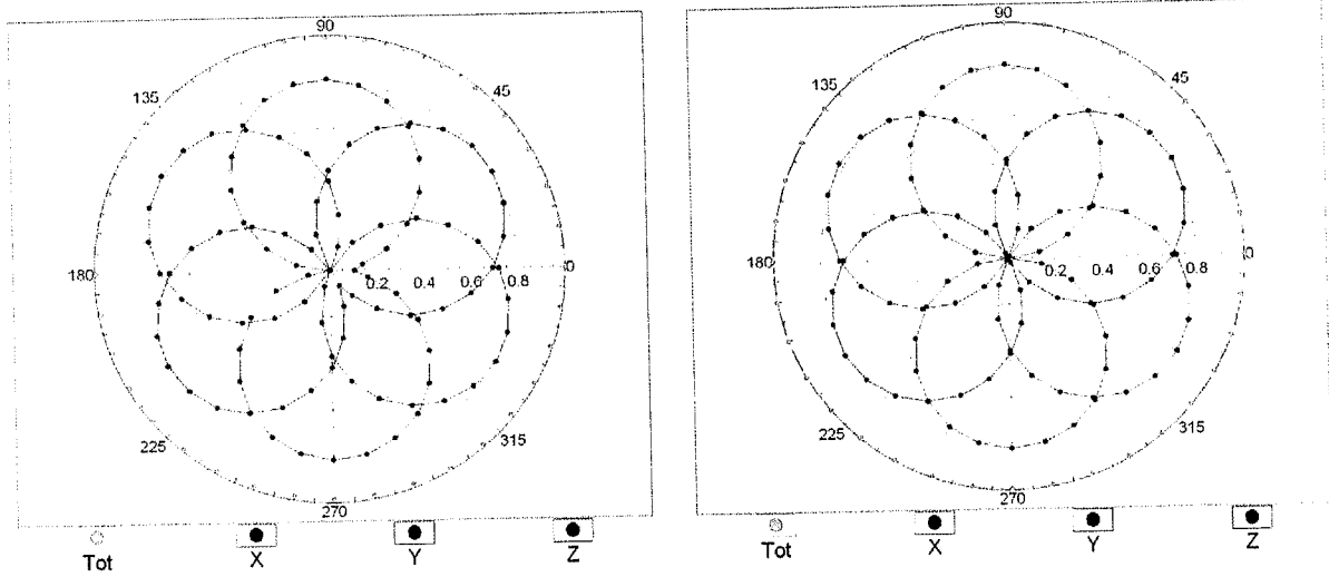
f=600 MHz,TEM
