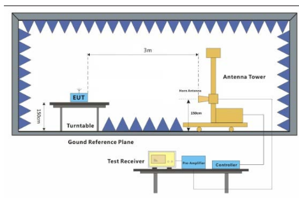
Figure 3. above 1GHz
