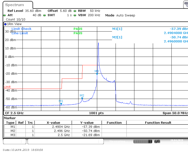
Band7_5MHz_64QAM_20775_25RB#0
