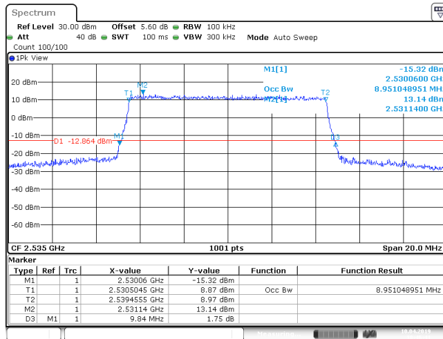
Band7_10MHz_16QAM_21400_50RB#
