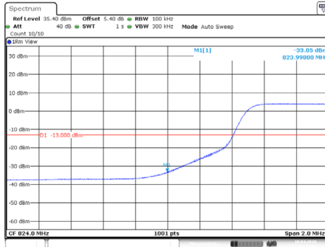
Band26_10MHz_QPSK_26840_50RB#0
