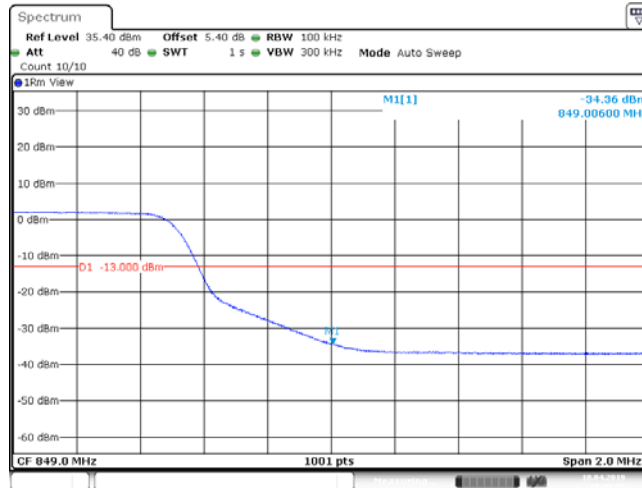
Band26_10MHz_16QAM_26990_50RB#0
