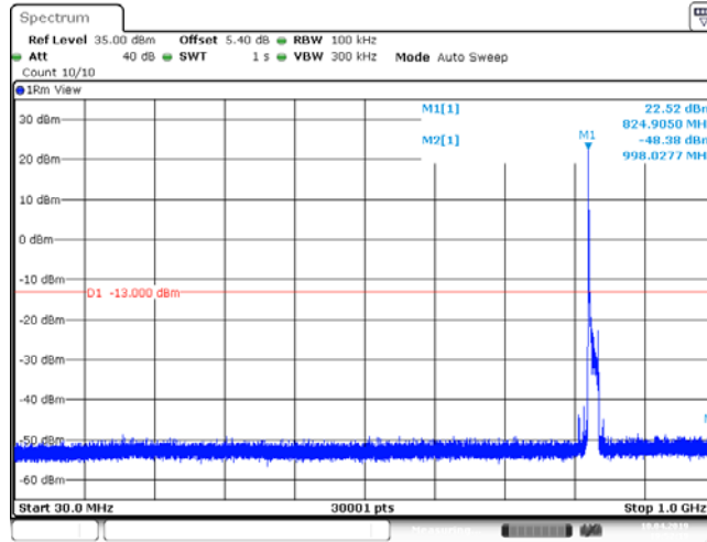
Band26_15MHz_QPSK_26865_1RB#0
