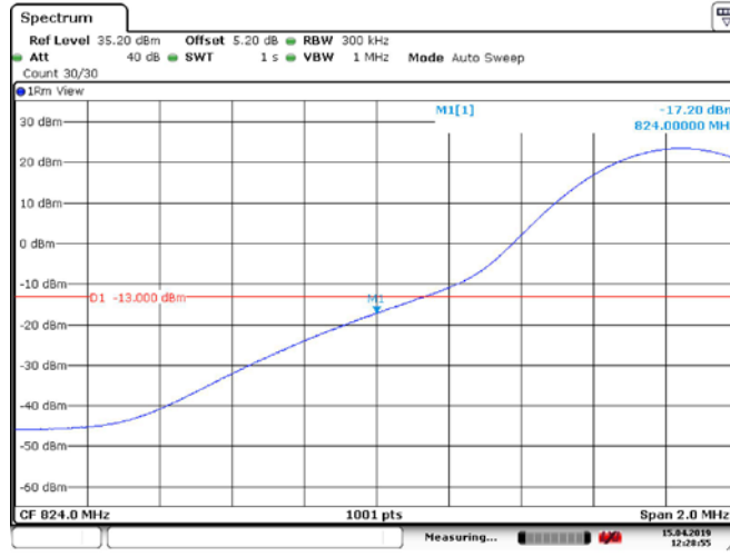
Band26_15MHz_QPSK_26865_50RB#0
