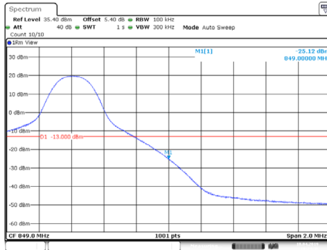
Band26_10MHz_64QAM_26990_50RB#0
