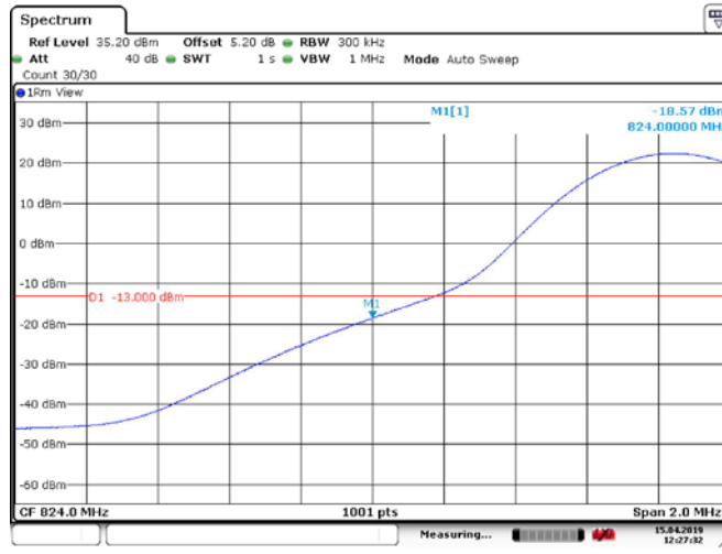
Band26_15MHz_16QAM_26865_50RB#0
