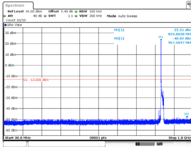
Band26_15MHz_QPSK_26965_1RB#0
