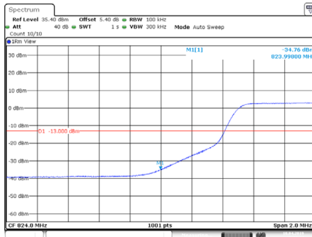
Band26_10MHz_64QAM_26840_50RB#0
