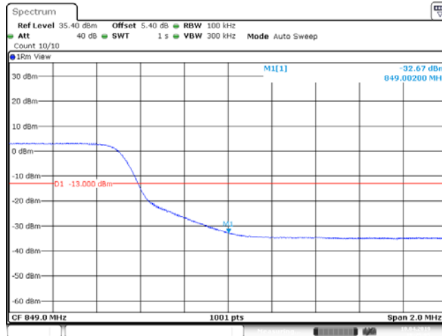
Band26_10MHz_QPSK_26990_50RB#0
