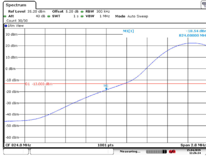
Band26_15MHz_64QAM_26865_50RB#0
