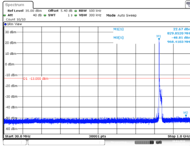
Band26_15MHz_QPSK_26915_1RB#0
