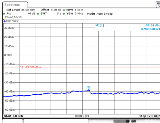
Band26_15MHz_QPSK_26965_1RB#0
