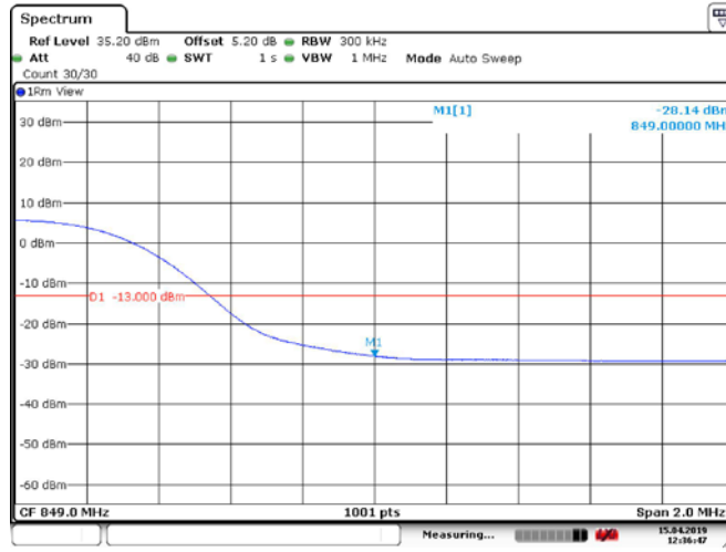
Band26_15MHz_QPSK_26965_50RB#0
