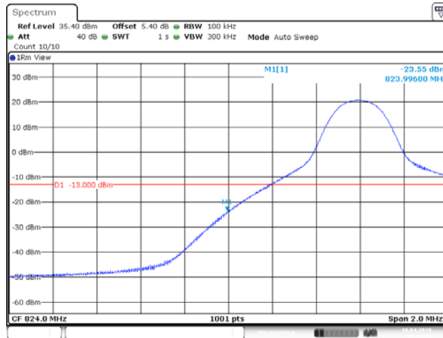
Band26_10MHz_64QAM_26840_50RB#0
