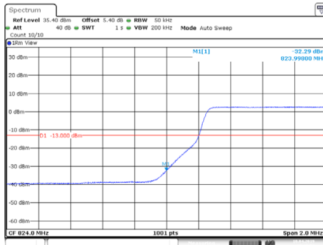
Band26_5MHz_64QAM_26815_25RB#0
