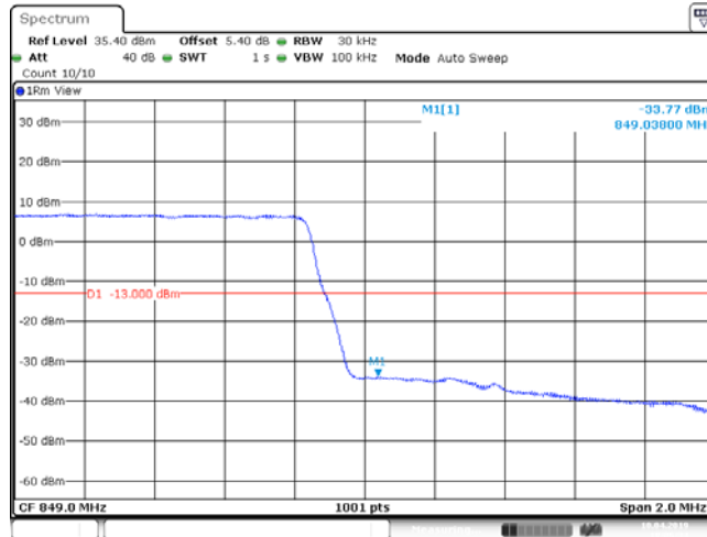
Band26_1.4MHz_64QAM_27033_6RB#0
