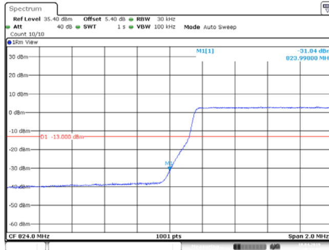
Band26_3MHz_16QAM_26805_15RB#0
