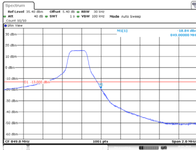
Band26_3MHz_64QAM_27025_15RB#0
