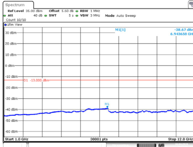
Band26_15MHz_64QAM_26915_1RB#0
