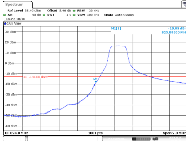
Band26_3MHz_QPSK_26805_15RB#0
