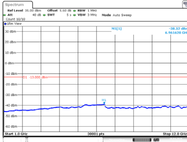
Band26_15MHz_16QAM_26915_1RB#0
