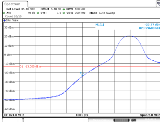
Band26_10MHz_16QAM_26840_50RB#0
