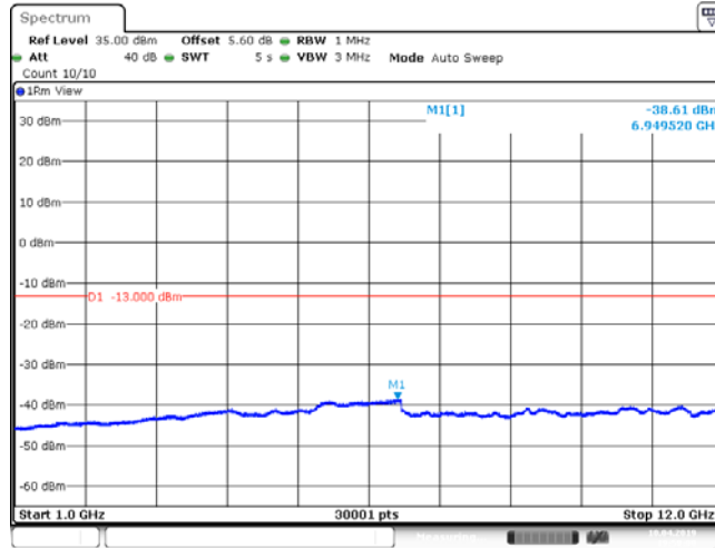
Band26_15MHz_QPSK_26915_1RB#0
