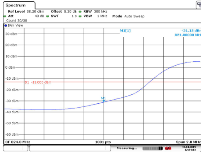
Band26_15MHz_16QAM_26865_50RB#0
