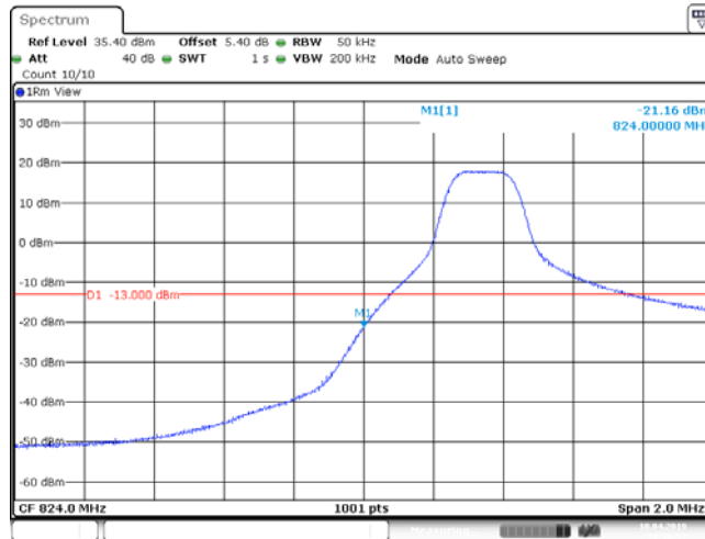
Band26_5MHz_64QAM_26815_25RB#0
