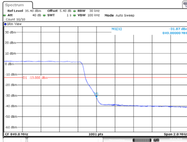
Band26_3MHz_64QAM_27025_15RB#0
