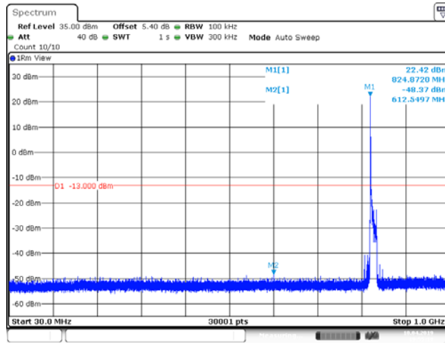
Band26_15MHz_64QAM_26865_1RB#0
