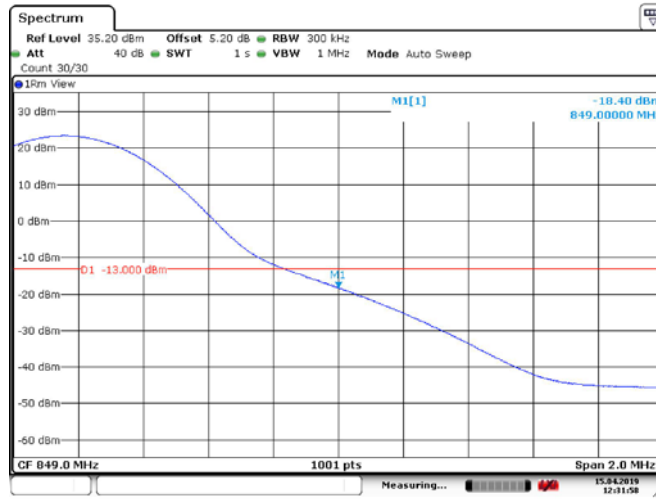
Band26_15MHz_QPSK_26965_50RB#0
