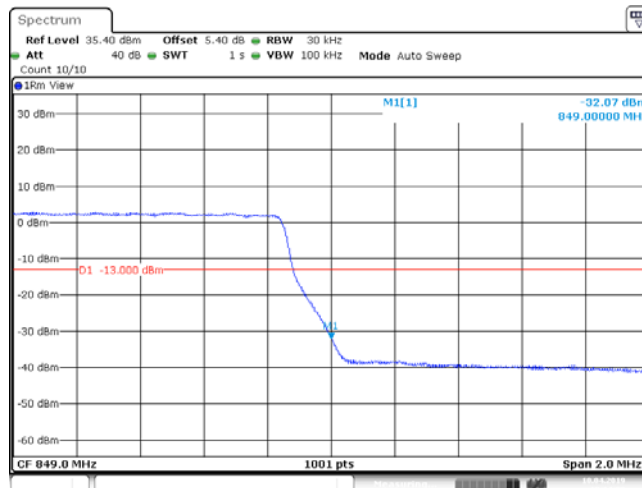
Band26_3MHz_16QAM_27025_15RB#0
