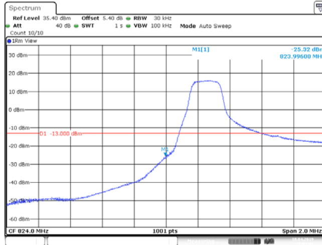
Band26_1.4MHz_16QAM_26767_6RB#0
