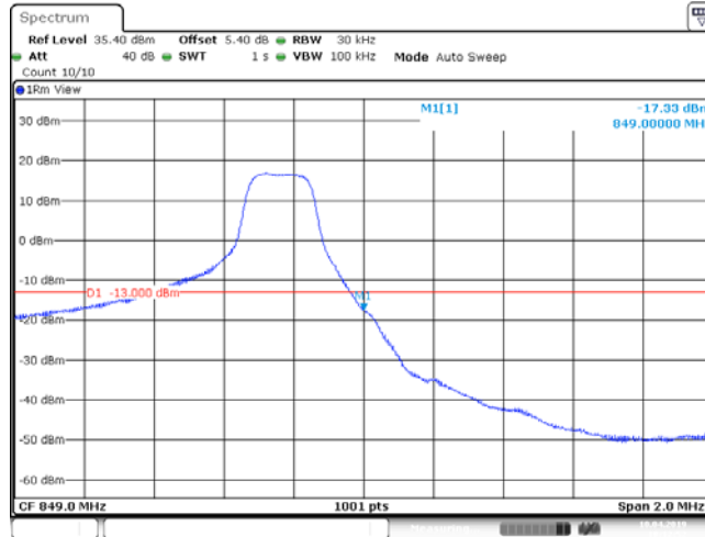
Band26_3MHz_QPSK_27025_15RB#0
