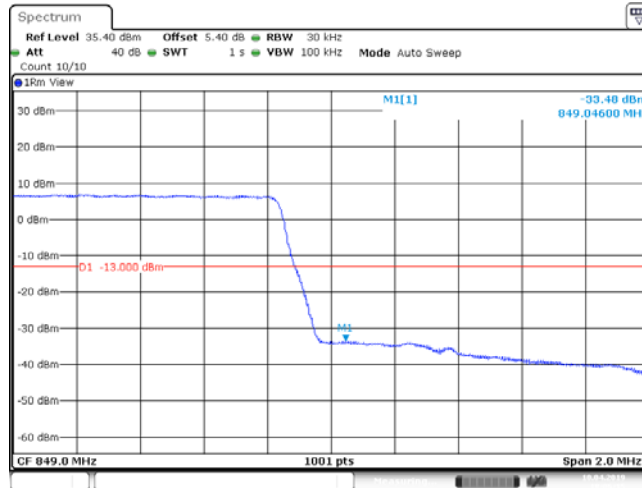
Band26_1.4MHz_16QAM_27033_6RB#0
