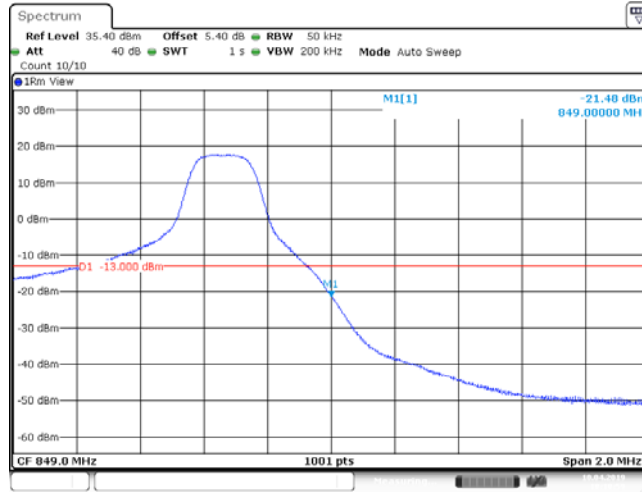
Band26_5MHz_64QAM_27015_25RB#0
