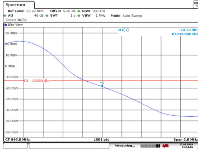
Band26_15MHz_64QAM_26965_50RB#0
