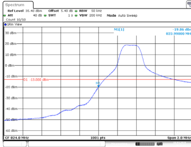
Band26_5MHz_QPSK_26815_25RB#0
