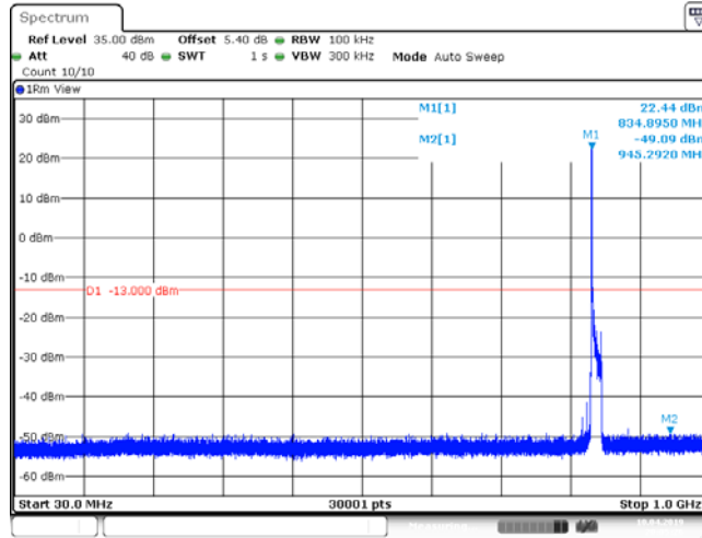
Band26_15MHz_64QAM_26965_1RB#0
