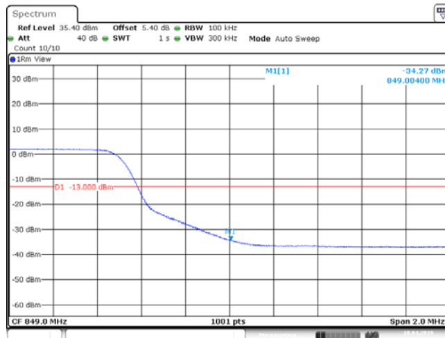
Band26_10MHz_64QAM_26990_50RB#0
