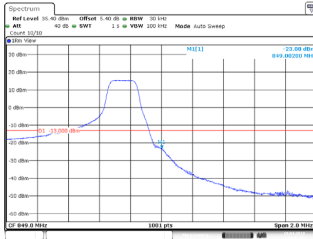
Band26_1.4MHz_64QAM_27033_6RB#0
