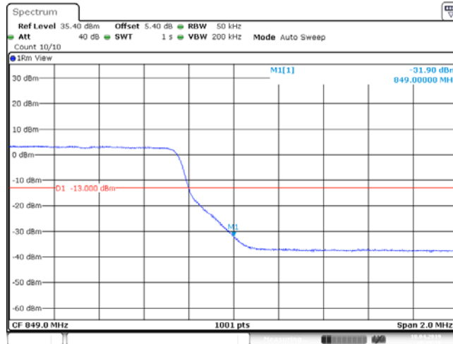
Band26_5MHz_QPSK_27015_25RB#0
