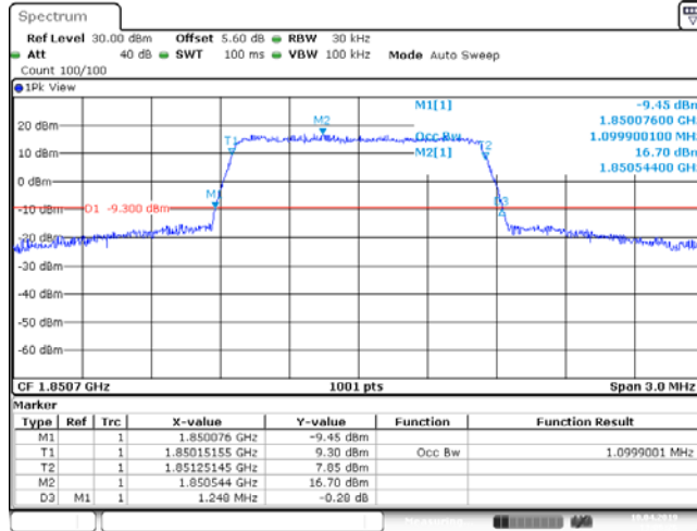
Band2_1.4MHz_64QAM_18607_6RB#0
