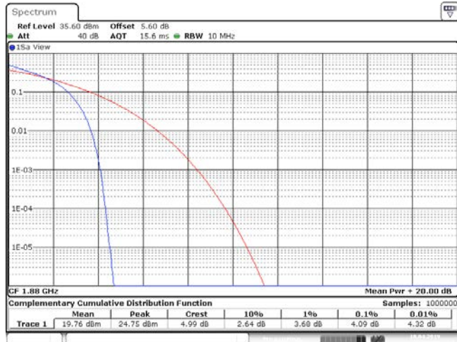
Band2_20MHz_64QAM_18900_100RB#0
