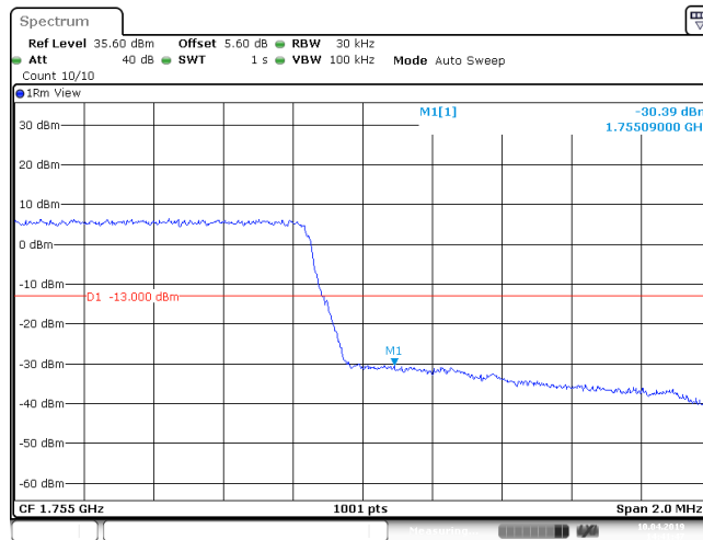
Band4_1.4MHz_64QAM_20393_6RB#0
