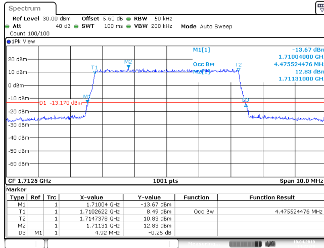
Band4_5MHz_64QAM_19975_25RB#0
