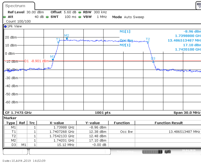
Band4_15MHz_64QAM_2025_75RB#0
