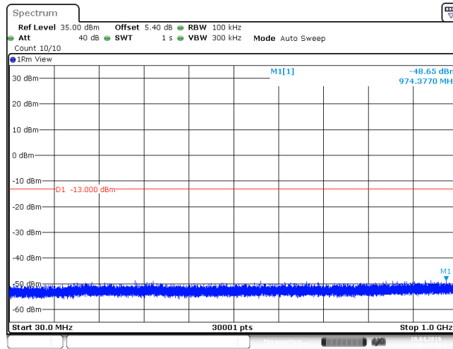
Band4_20MHz_QPSK_20300_1RB#0
