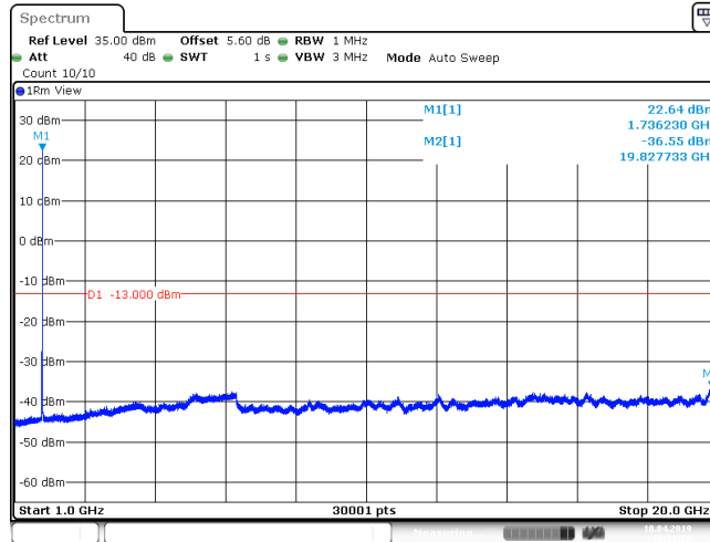
Band4_20MHz_64QAM_20300_1RB#0
