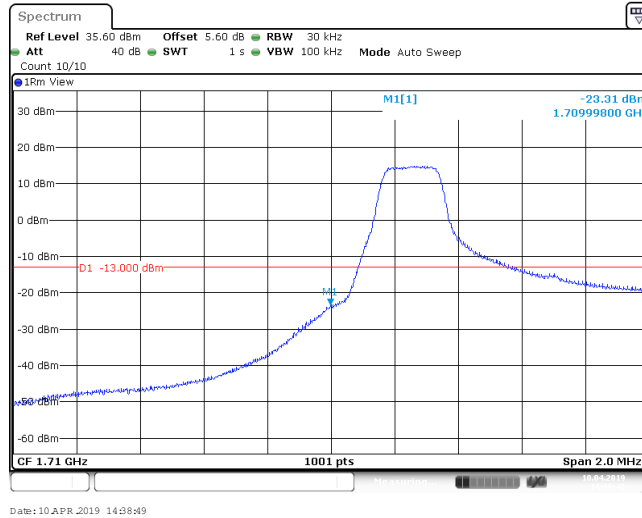
Band4_1.4MHz_64QAM_19957_6RB#0
