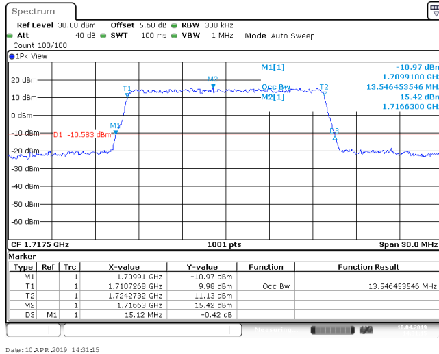
Band4_15MHz_64QAM_20175_75RB#0
