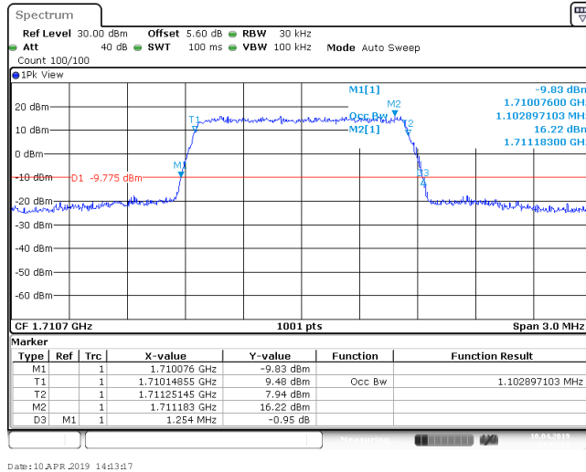
Band4_1.4MHz_64QAM_20175_6RB#0
