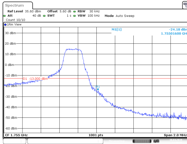
Band4_1.4MHz_64QAM_20393_6RB#0
