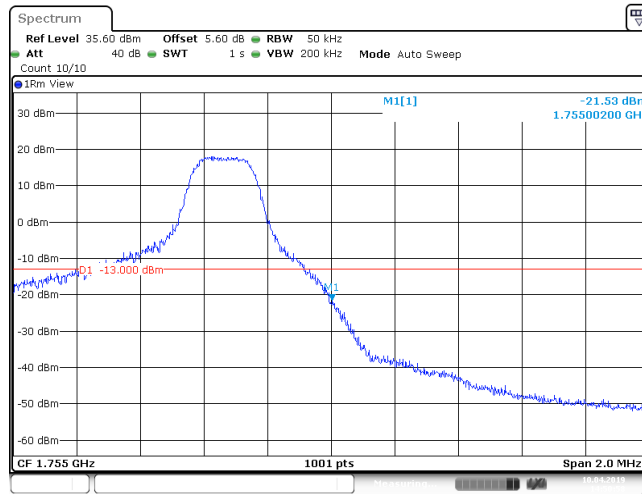
Band4_5MHz_QPSK_20375_25RB#0
