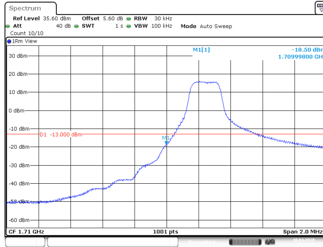
Band4_3MHz_QPSK_19965_15RB#0
