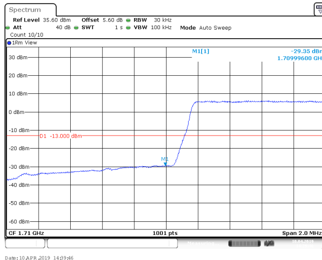
Band4_1.4MHz_64QAM_20393_1RB#5
