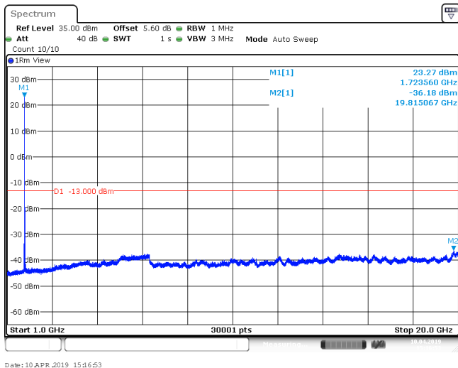
Band4_20MHz_64QAM_20300_1RB#0
