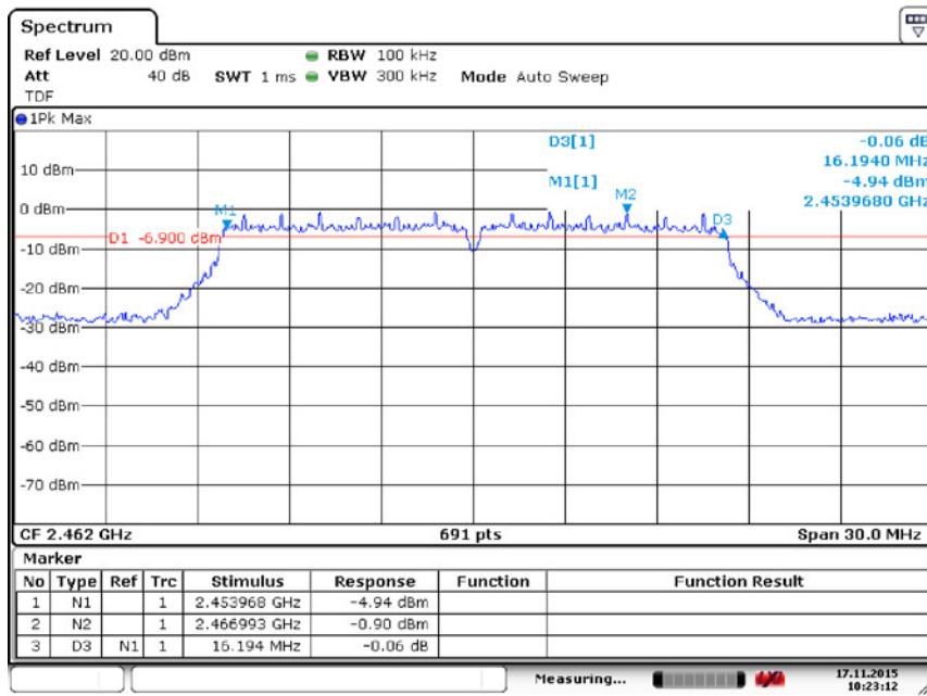
Fig.75 Occupied 6dB Bandwidth (802.11g, Ch 11)
