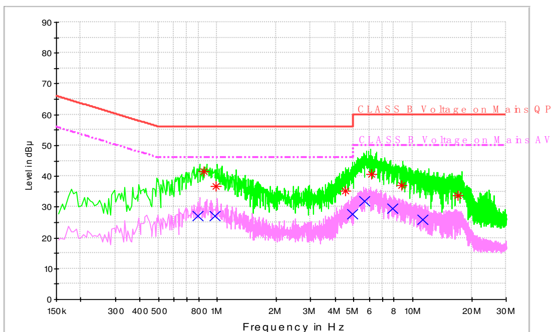
CLASS B Voltage with ENV216
