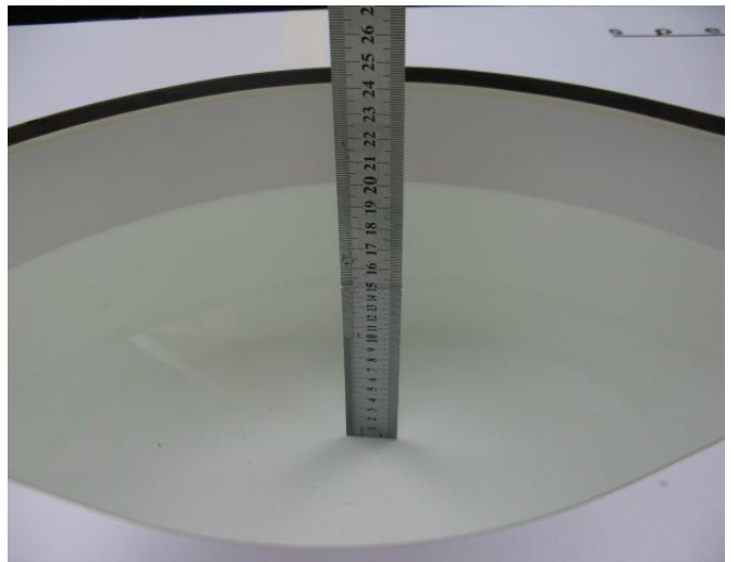
Photo 21: MSL1900MHz depth (15.2cm)
