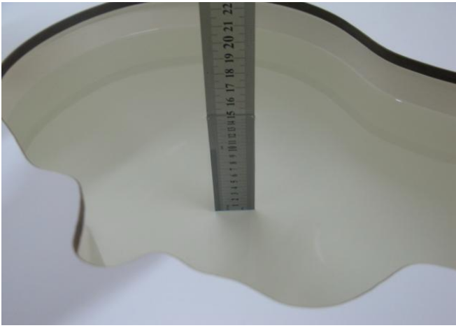
Photo 22: HSL2450MHz depth (15.0cm)
