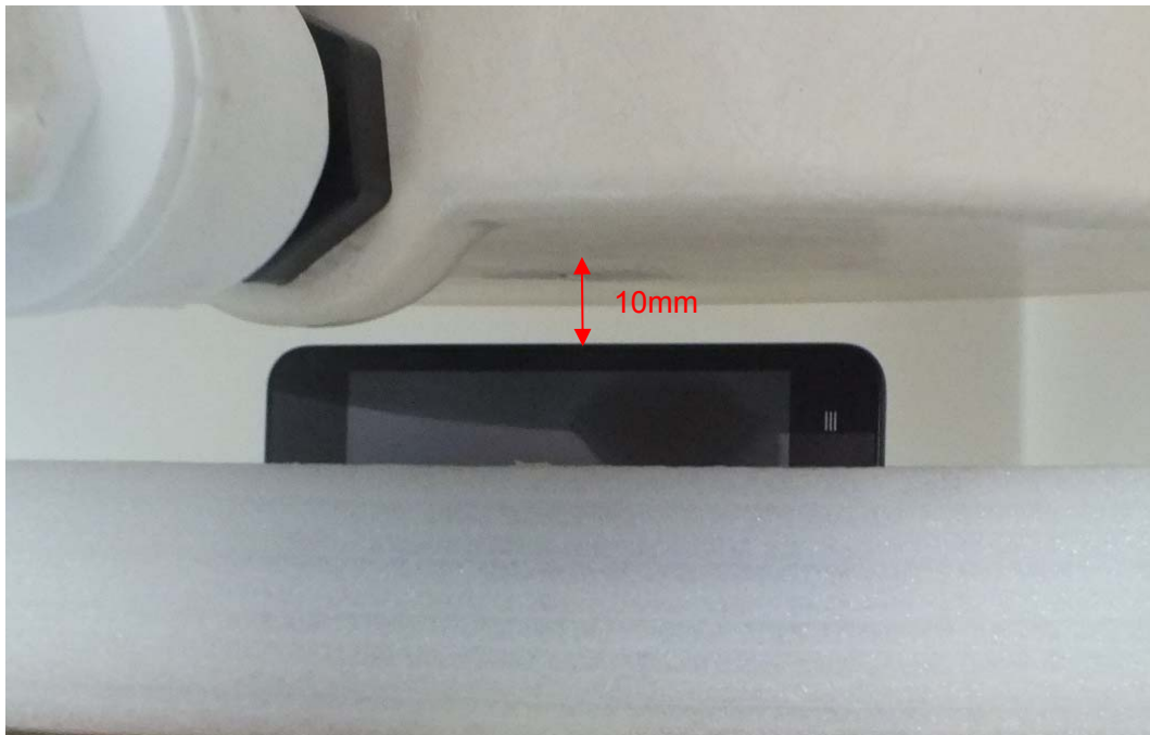
Picture 16: Right Edge, the distance from handset to the bottom of the Phantom is 10mm
