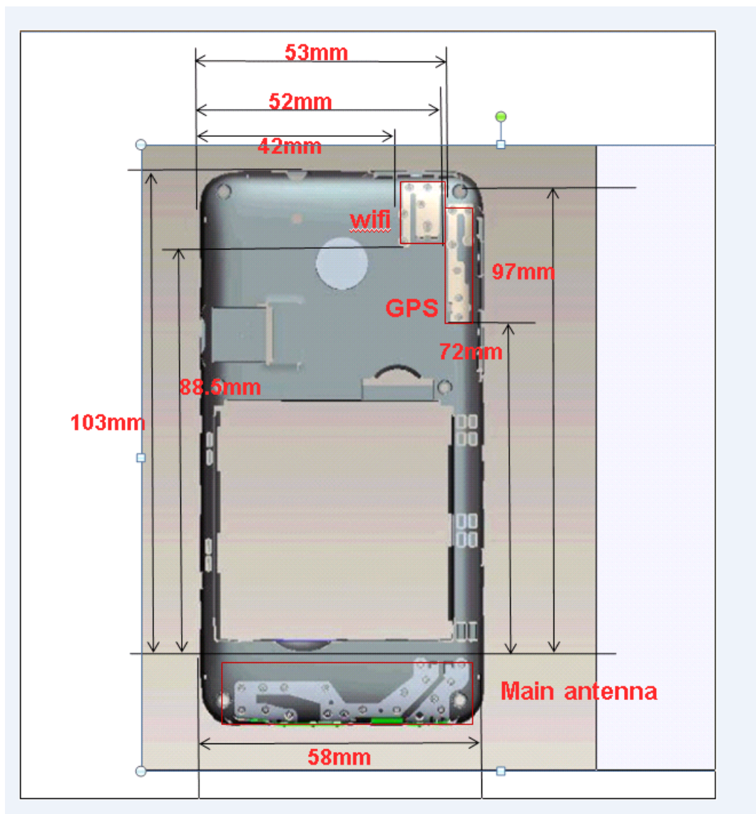
Picture 8: Constituents of EUT
