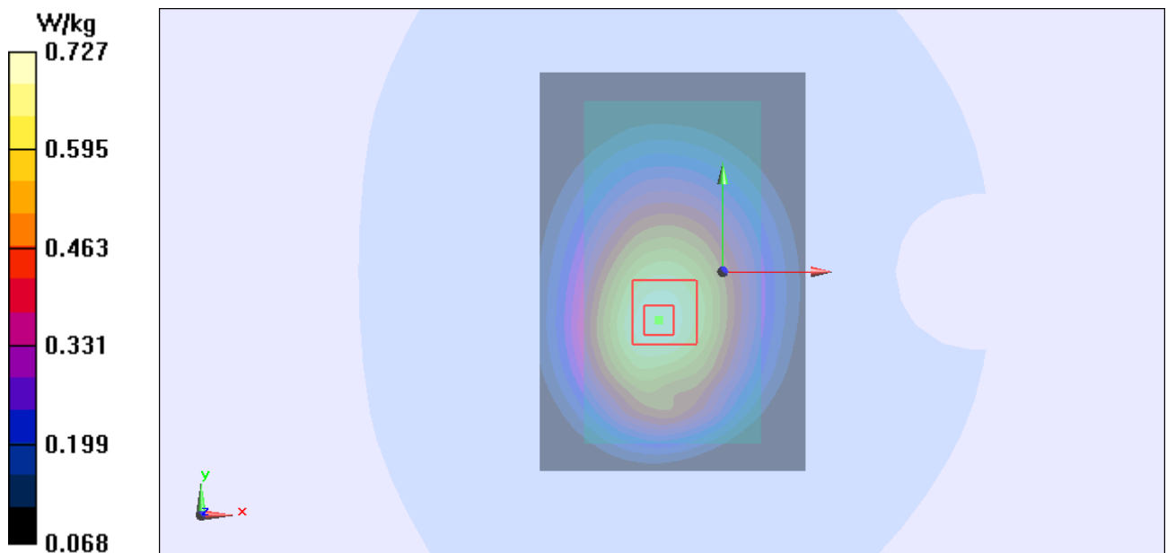
Figure 103 Body, Back Side, UMTS Band V Channel 4183
