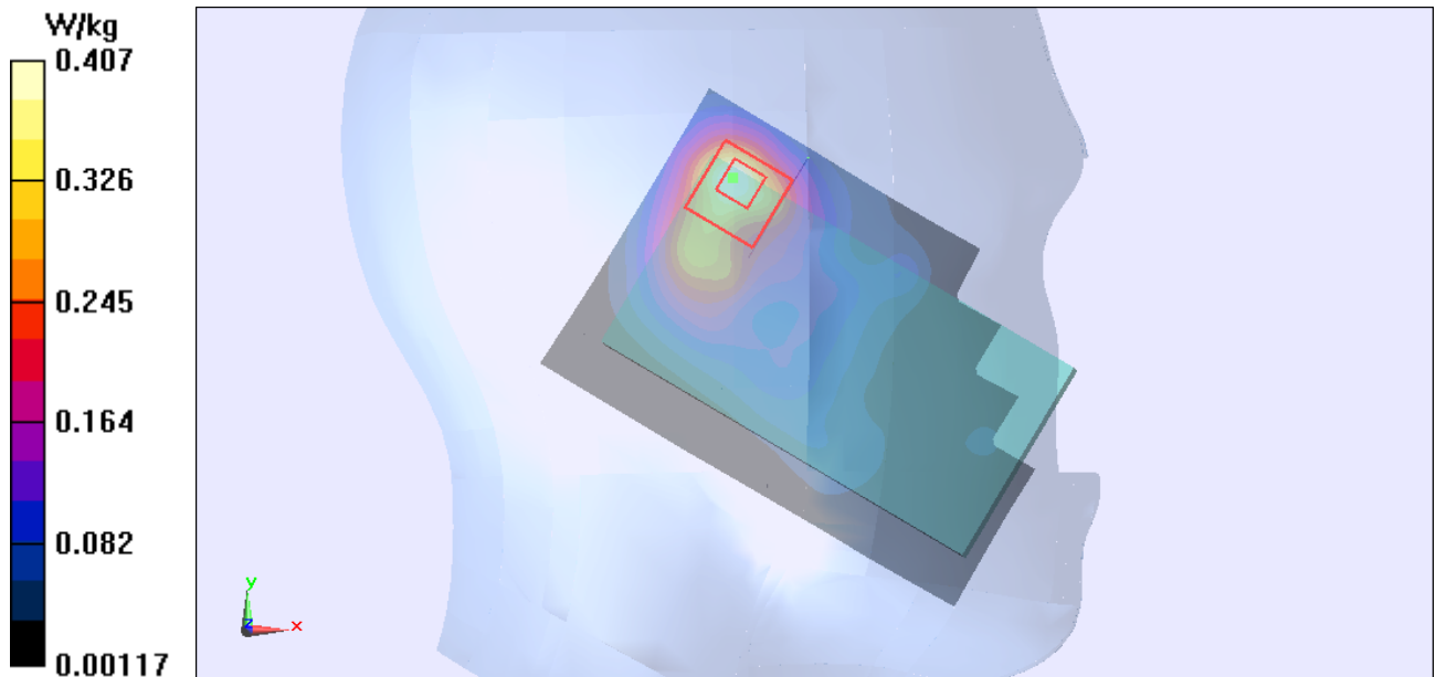
Figure 104 Left Hand Touch Cheek 802.11b Channel 11
