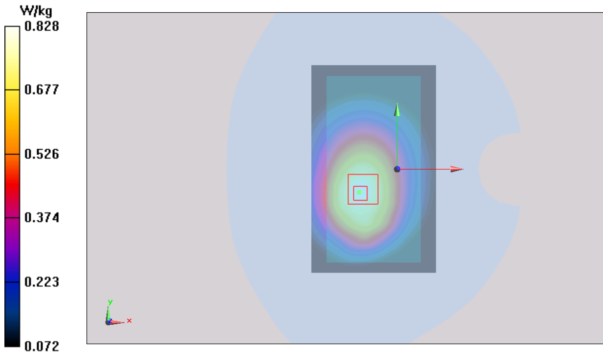
Figure 132 Body, Back Side, UMTS Band V Channel 4183
