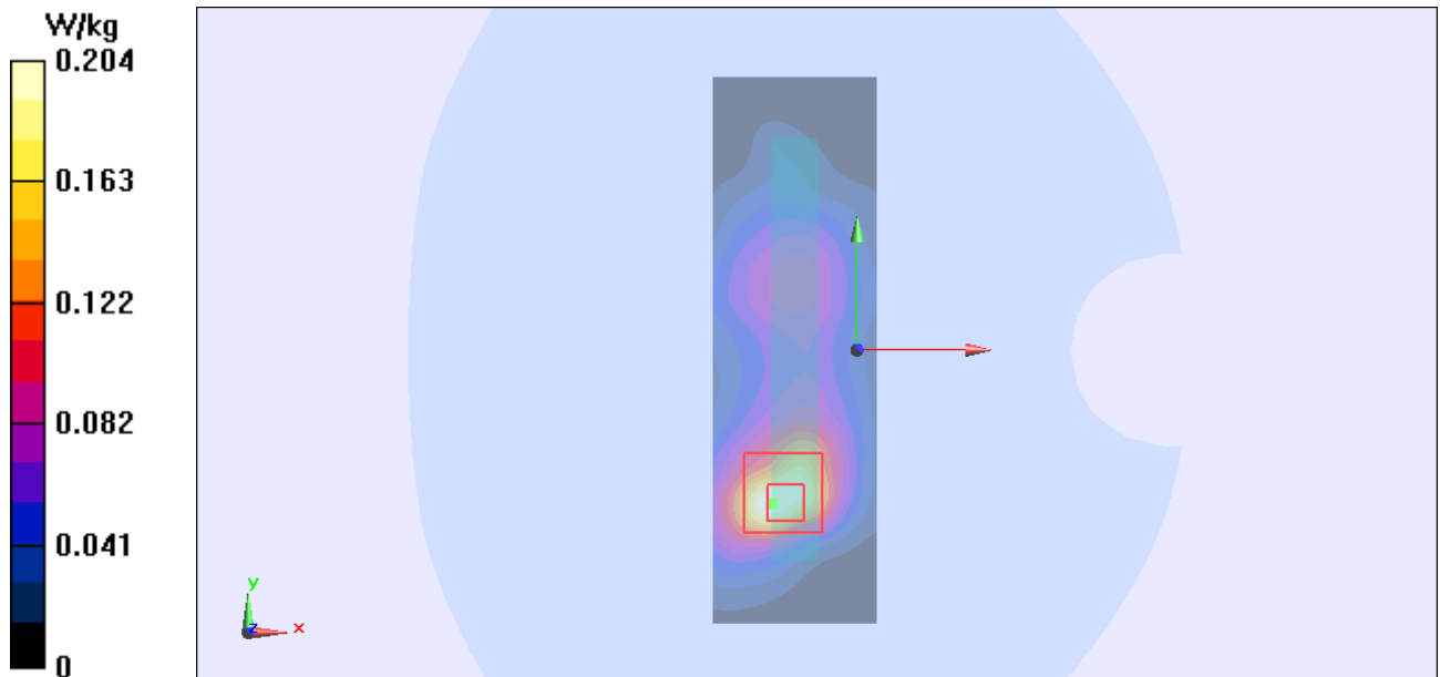
Figure 113 Body, Right Edge, 802.11b Channel 11
