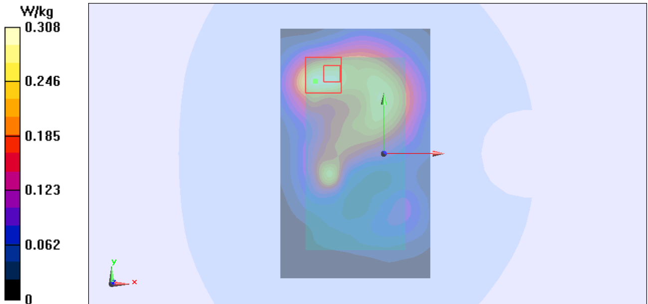
Figure 117 Body, Back Side, 802.11b Channel 11
