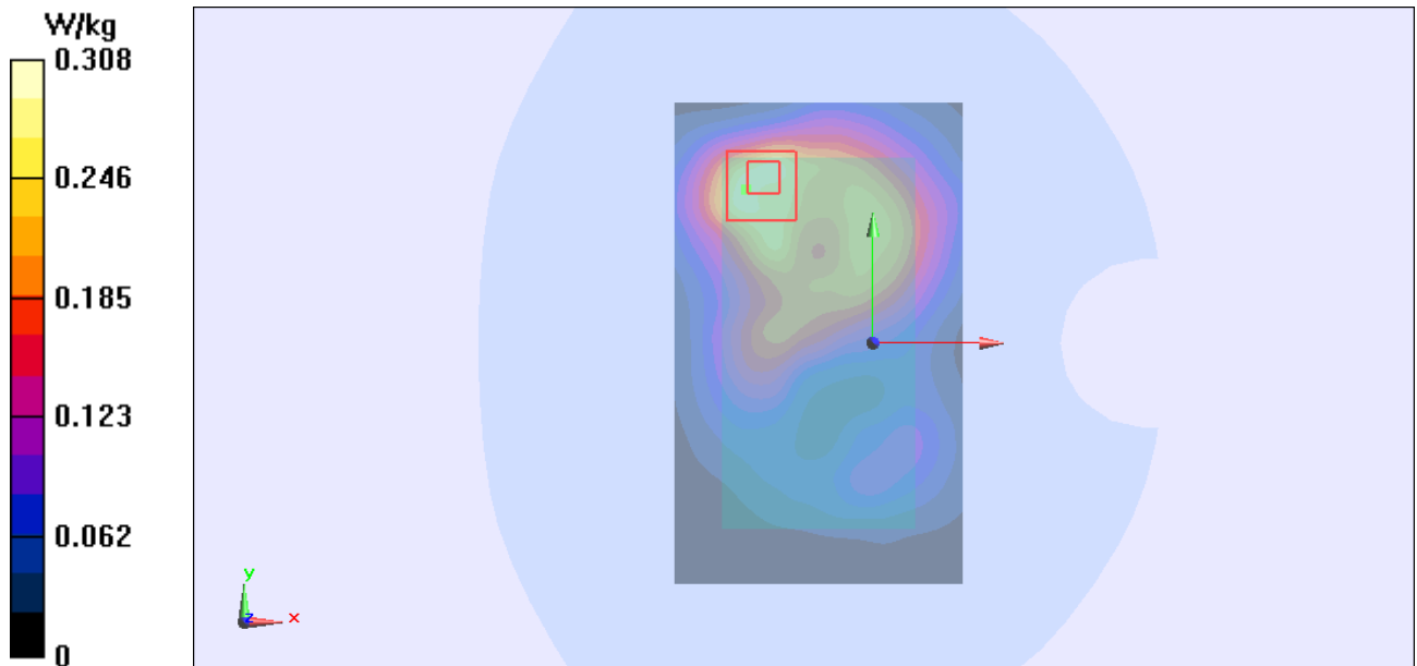
Figure 116 Body, Back Side, 802.11b Channel 11
