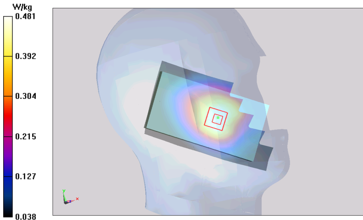
Figure 131 Left Touch Cheek UMTS Band V Channel 4183
