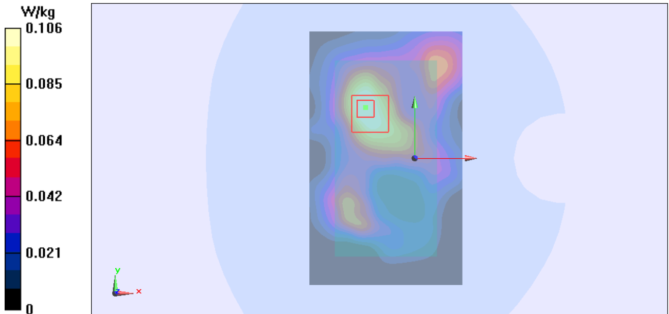
Figure 112 Body, Front Side, 802.11b Channel 11
