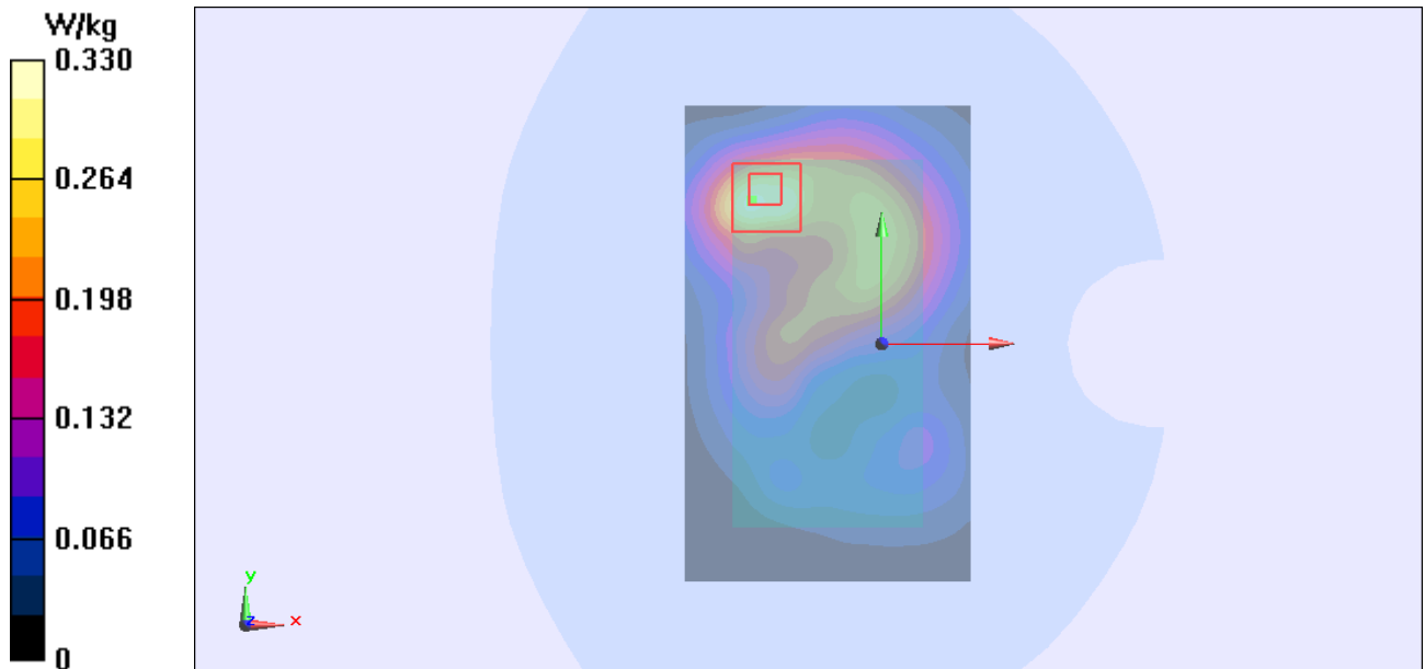
Figure 115 Body, Back Side, 802.11b Channel 11
