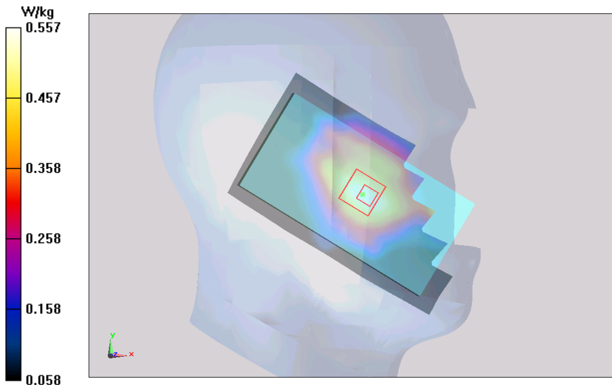
Figure 122 Left Hand Touch Cheek GSM 850 Channel 190
