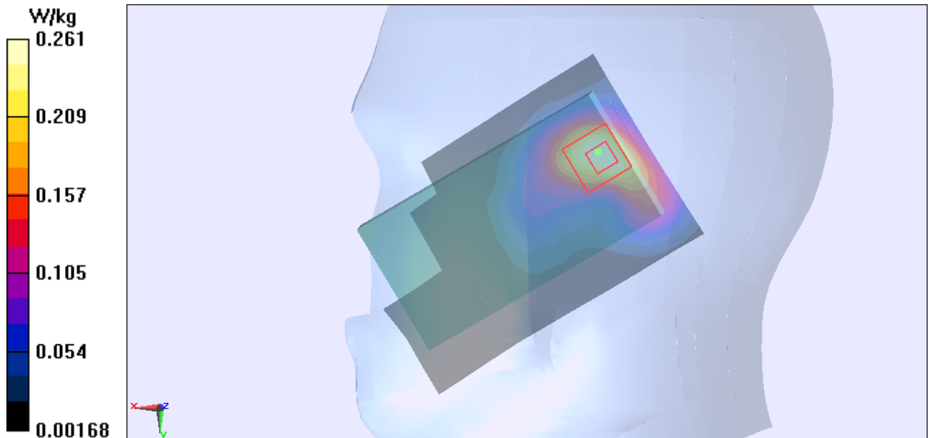
Figure 107 Right Hand Tilt 15° 802.11b Channel 11
