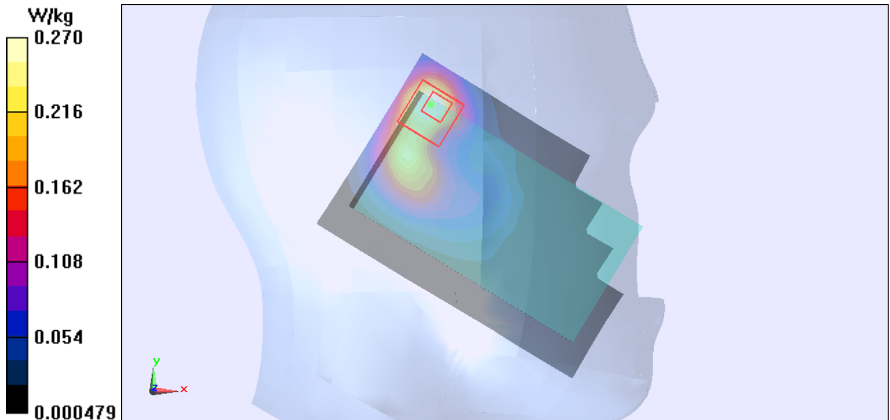
Figure 105 Left Hand Tilt 15° 802.11b Channel 11
