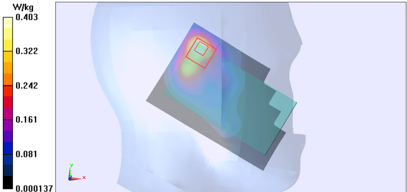
Figure 108 Left Hand Touch Cheek 802.11b Channel 11
