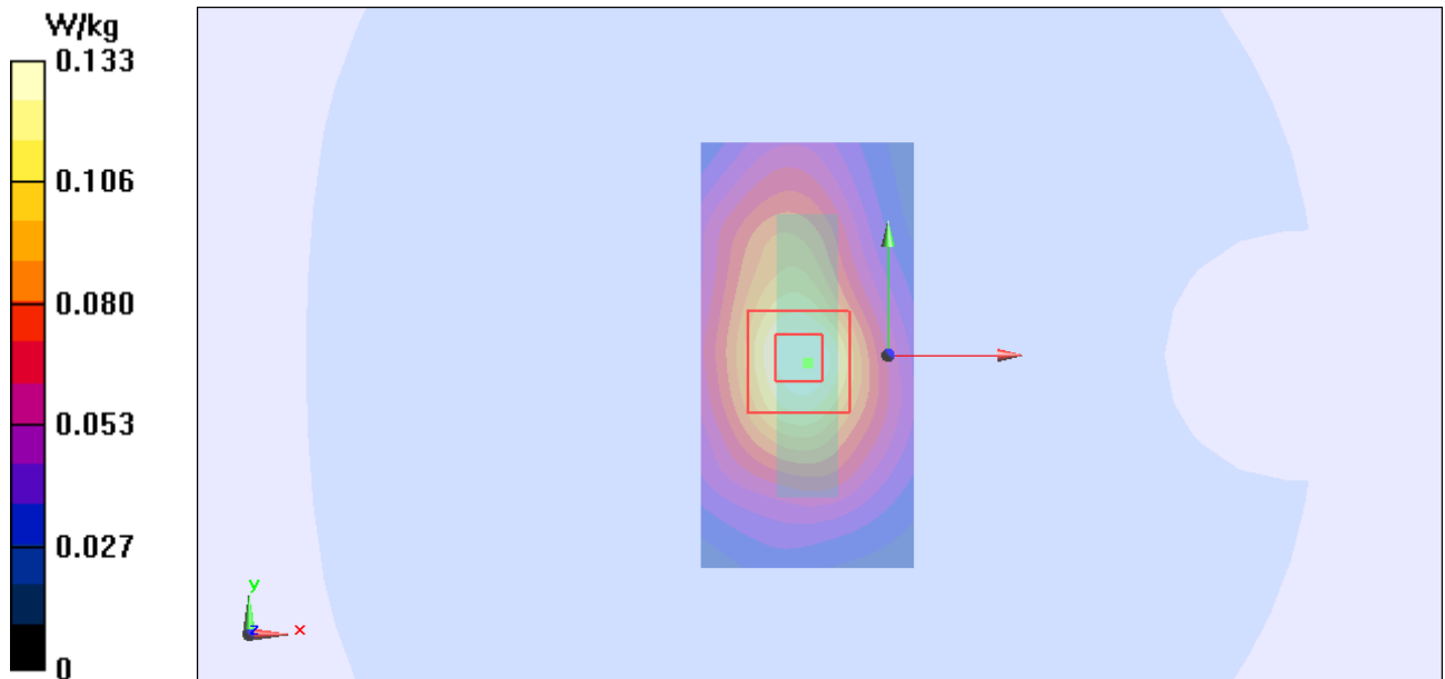
Figure 114 Body, Top Edge, 802.11b Channel 11
