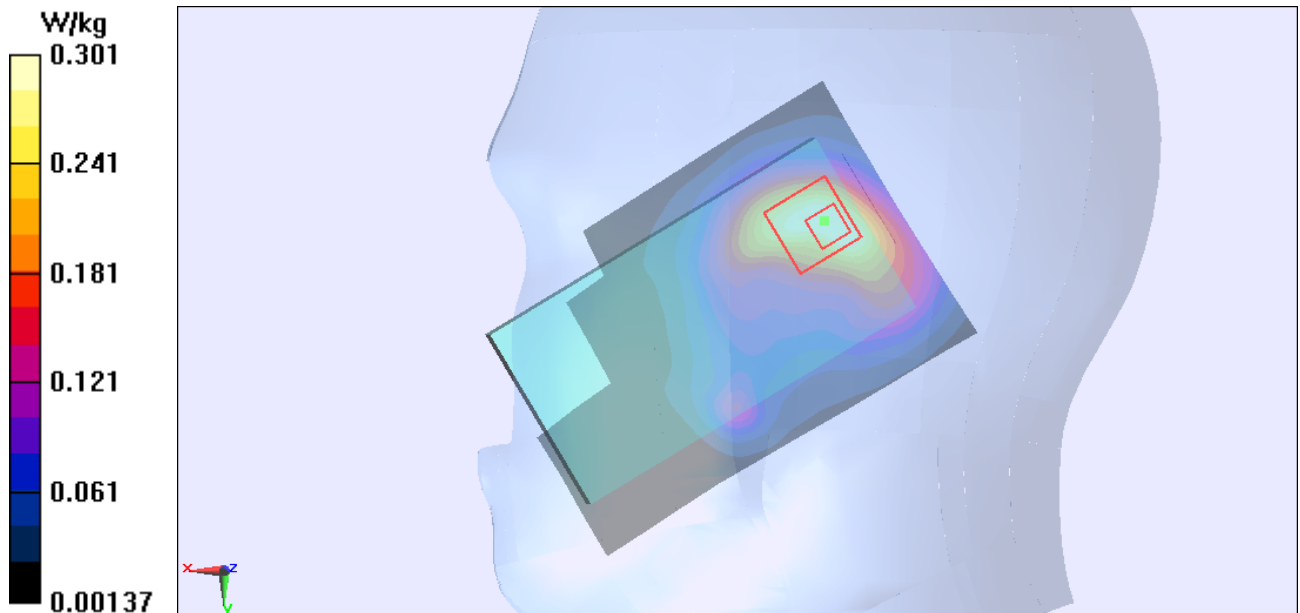
Figure 106 Right Hand Touch Cheek 802.11b Channel 11
