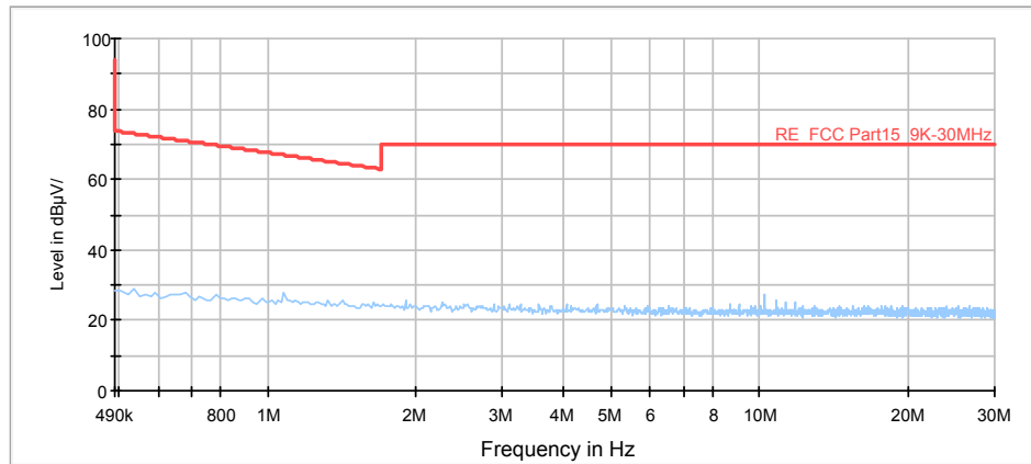
Radiates Emission from 490KHz to 30MHz
