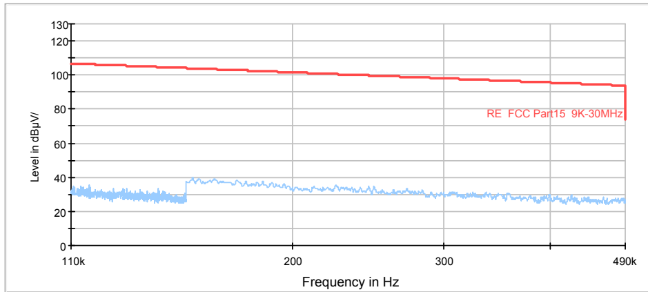
Radiates Emission from 110KHz to 490KHz
