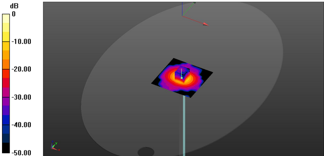
0 dB = 19.7 W/kg
