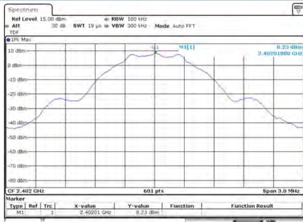
GFSK (BLE) LOW CHANNEL , CARRIER LEVEL
