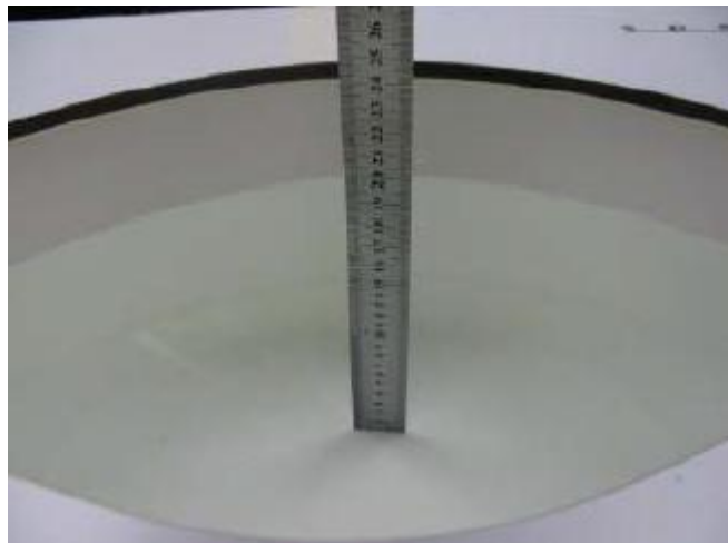
Photo 28: MBBL 3500-5800MHz depth (15.1cm)
