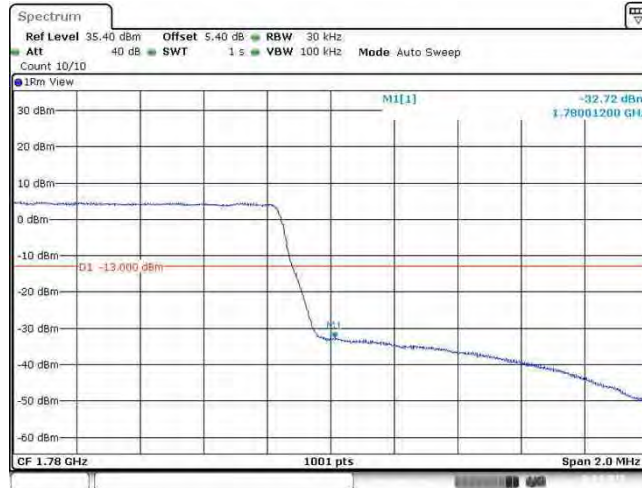
Band66_1.4MHz_64QAM_132665_6RB#
