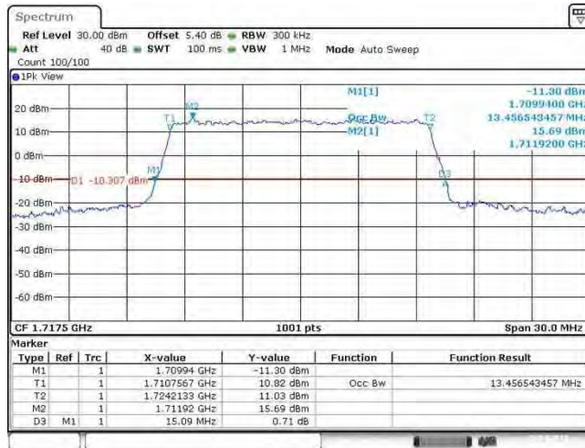
Band66_15MHz_QPSK_132322_75RB#0
