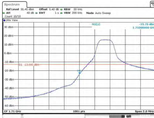
Band66_5MHz_16QAM_131997_25RB#0
