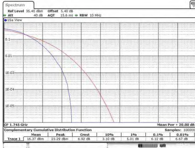
Band66_20MHz_64QAM_132322_100RB#0
