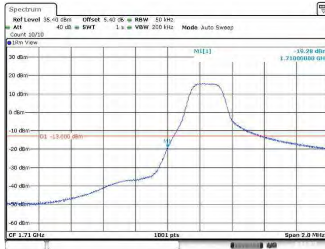
Band66_3MHz_16QAM_131987_15RB#0
