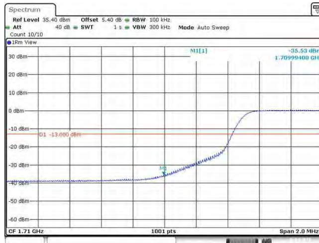
Band66_10MHz_64QAM_132022_50RB#0
