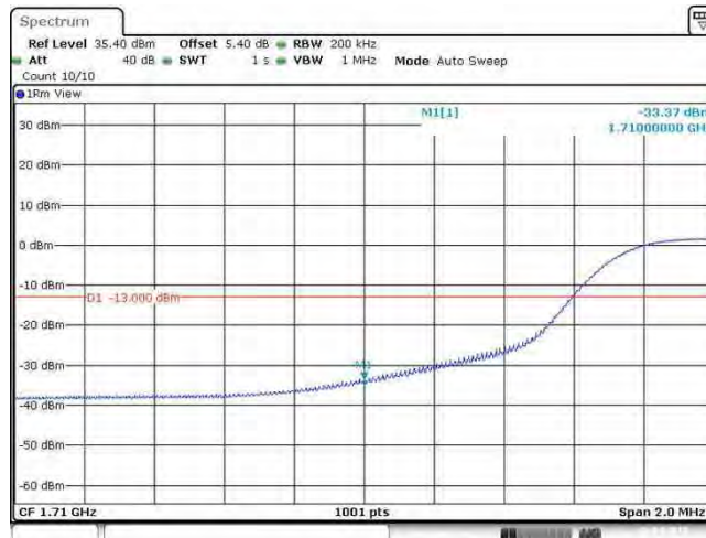
Band66_15MHz_16QAM_132047_75RB#0
