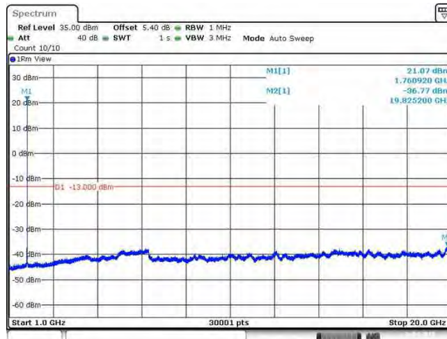
Band66_20MHz_64QAM_132572_1RB#0
