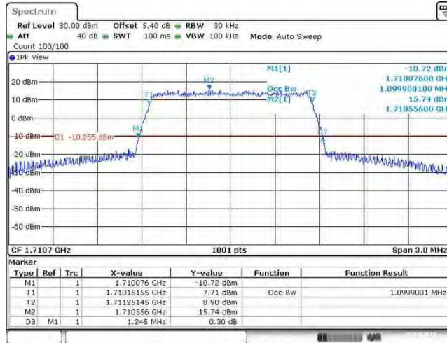
Band66_1.4MHz_64QAM_131979_6RB#0
