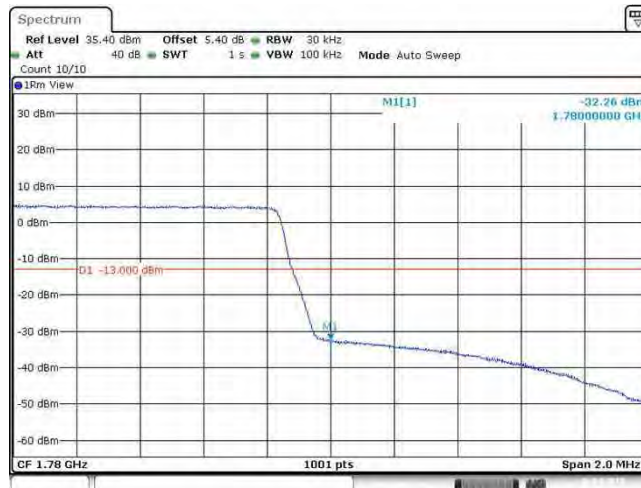
Band66_1.4MHz_16QAM_132665_6RB#0
