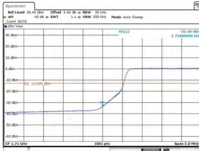
Band66_5MHz_16QAM_131997_25RB#0
