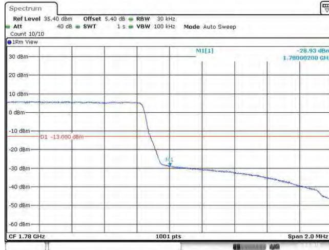
Band66_1.4MHz_QPSK_132665_6RB#0
