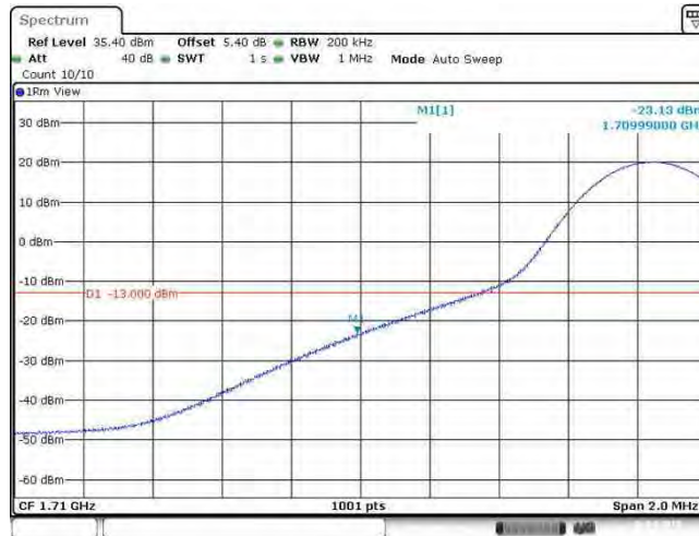
Band66_15MHz_16QAM_132047_75RB#0
