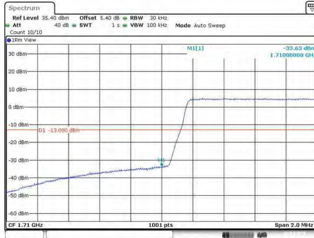
Band66_1.4MHz_64QAM_131979_6RB#0
