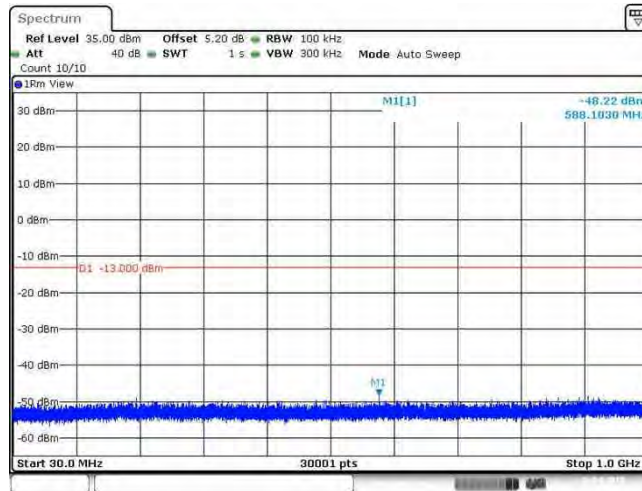
Band66_20MHz_64QAM_132572_1RB#0
