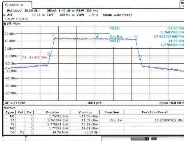
Band66_20MHz_QPSK_132572_100RB#0
