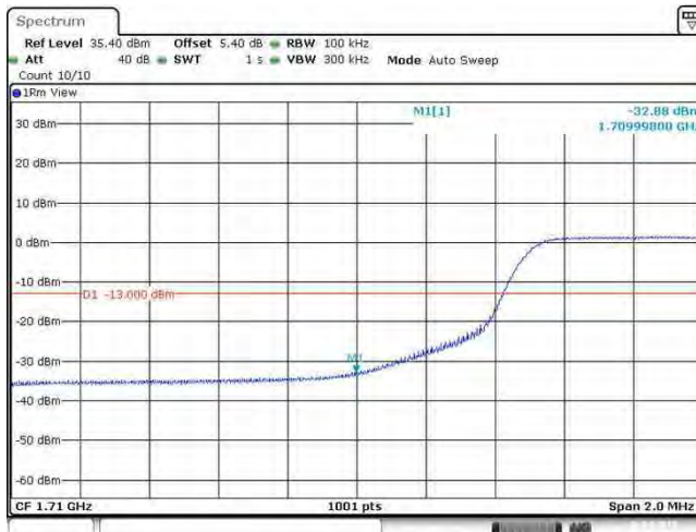
Band66_10MHz_QPSK_132022_50RB#0
