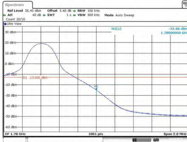
Band66_10MHz_QPSK_132622_50RB#0
