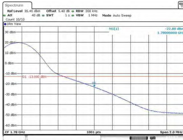
Band66_15MHz_16QAM_132597_75RB#0
