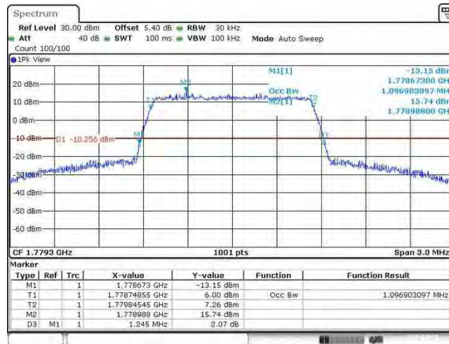
Band66_1.4MHz_64QAM_132665_6RB#0
