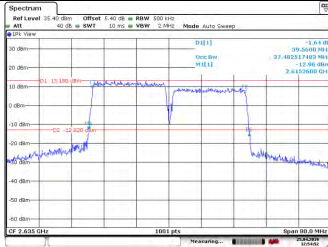
CA_41C_64QAM_100RB+100RB_40338+40140_PCC:100RB@0_SCC:100RB@0
