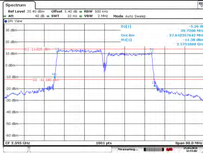
CA_41C_QPSK_100RB+100RB_40541+40739_PCC:100RB@0_SCC:100RB@0
