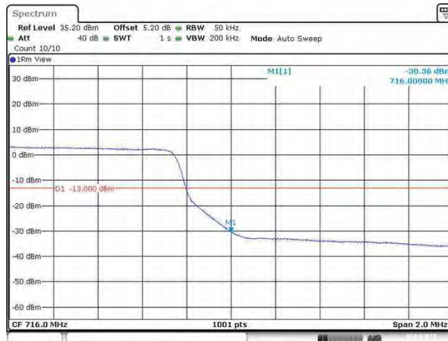
Band12_5MHz_QPSK_23155_25RB#0
