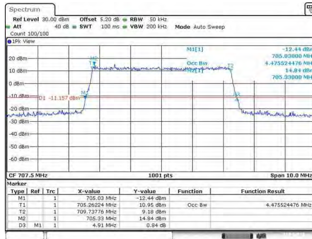
Band12_5MHz_16QAM_23095_25RB#0
