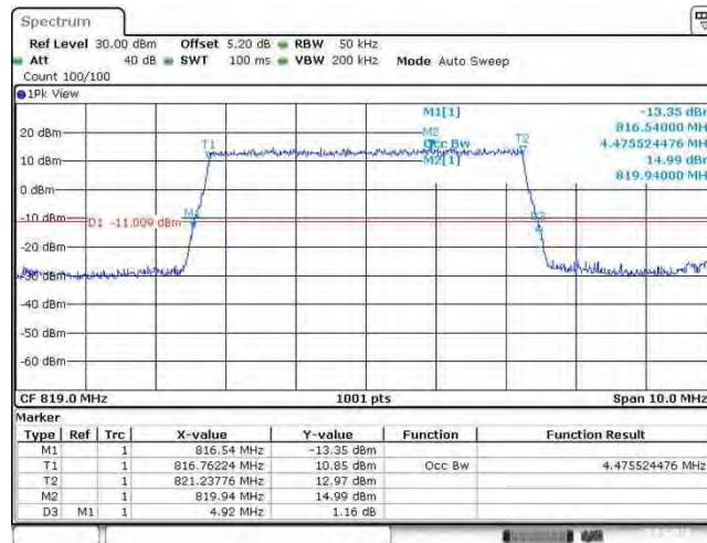
Band26_5MHz_QPSK_26740_25RB#0
