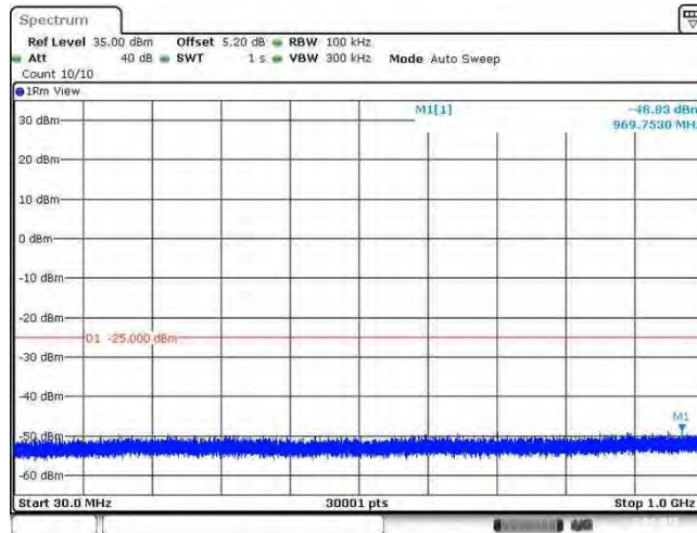
Band41_20MHz_16QAM_40640_1RB#0
