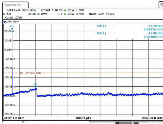
Band41_20MHz_16QAM_40640_1RB#0
