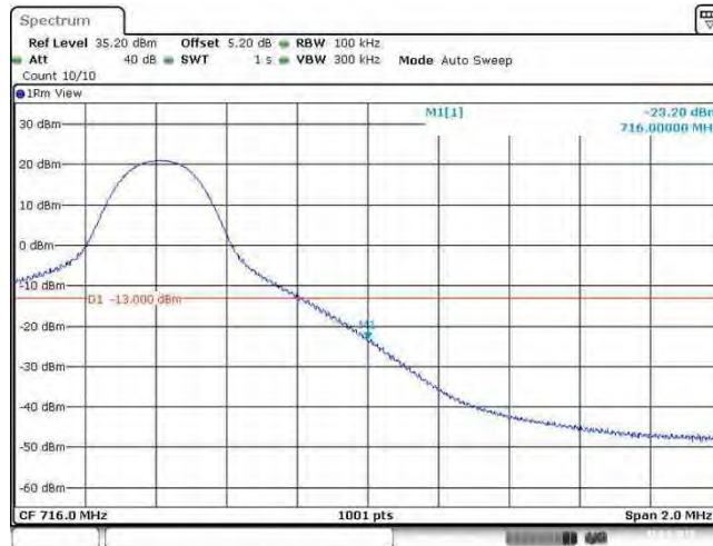
Band17_10MHz_64QAM_23800_50RB#0
