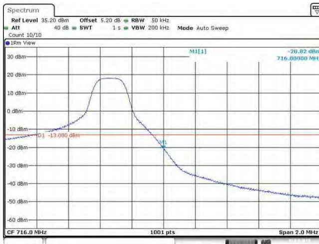
Band17_5MHz_64QAM_23825_25RB#0
