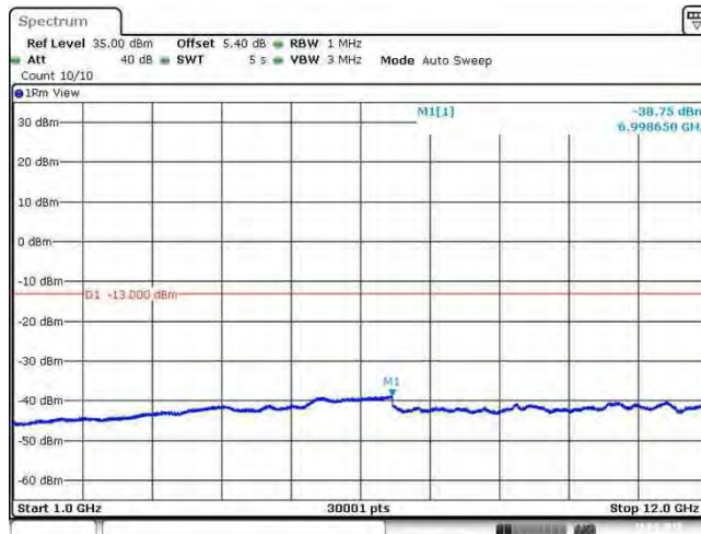
Band17_10MHz_64QAM_23800_1RB#0
