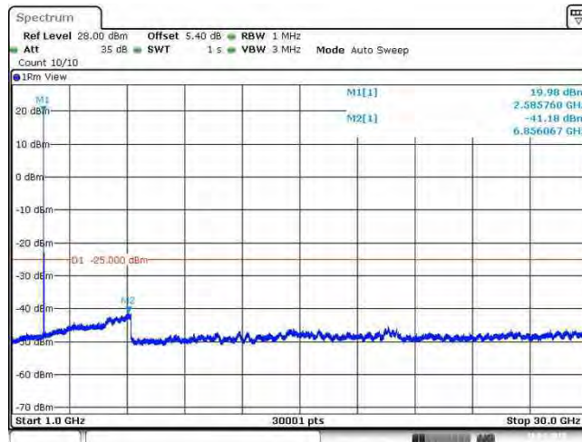
Band38_20MHz_64QAM_38000_1RB#0
