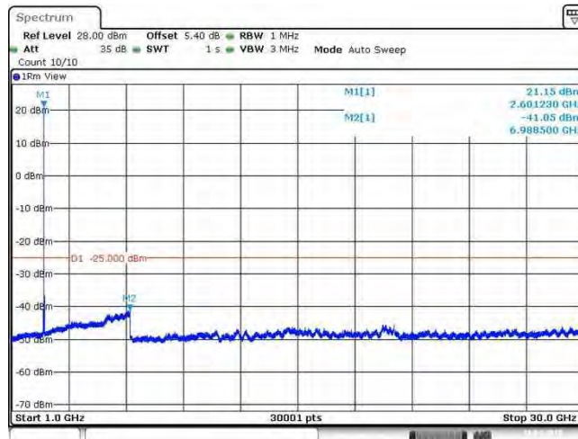
Band38_20MHz_64QAM_38150_1RB#0
