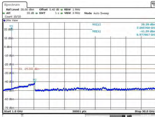
Band38_20MHz_16QAM_38000_1RB#0
