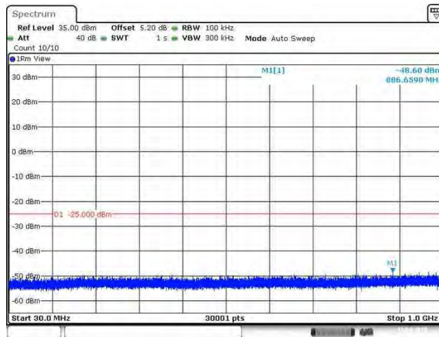
Band38_20MHz_QPSK_38000_1RB#0
