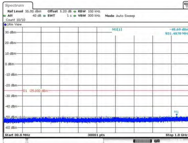
Band38_20MHz_64QAM_38000_1RB#0
