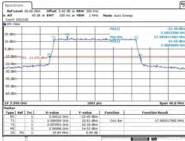
Band38_20MHz_QPSK_38150_100RB#0
