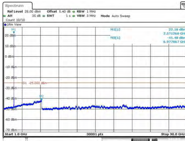
Band38_20MHz_16QAM_37850_1RB#0
