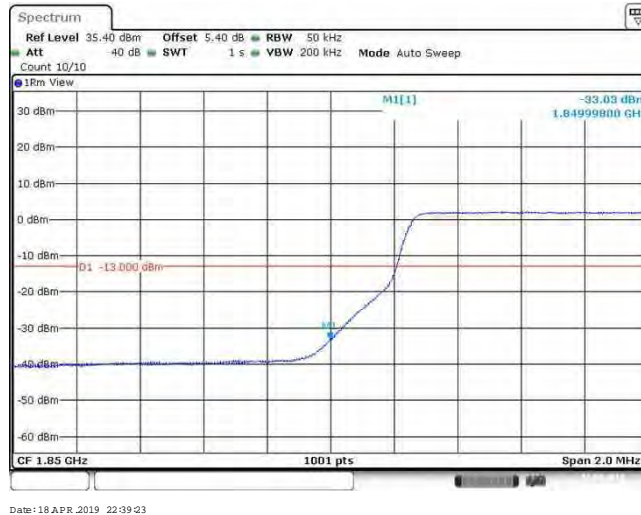
Band2_5MHz_64QAM_19175_1RB#24
