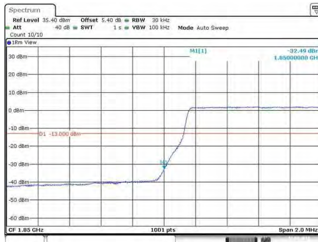
Band2_3MHz_64QAM_18615_15RB#0
