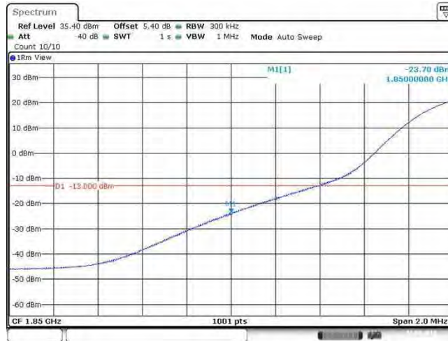
Band2_20MHz_64QAM_18700_100RB#0
