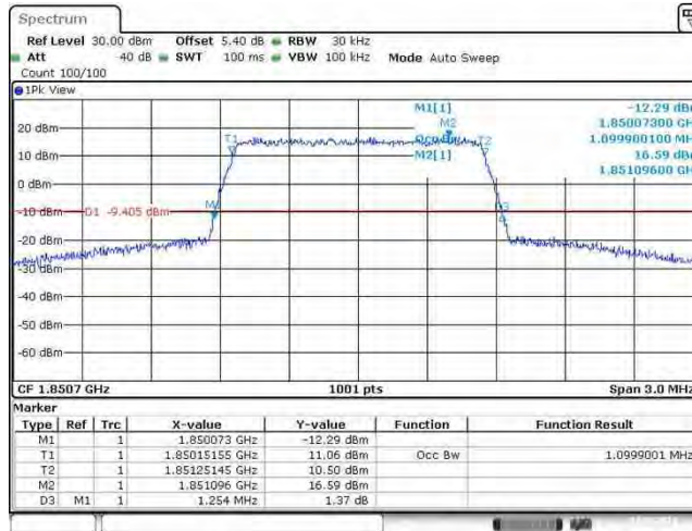
Band2_1.4MHz_QPSK_18607_6RB#0
