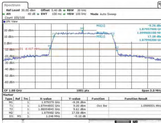
Band2_1.4MHz_QPSK_18900_6RB#0
