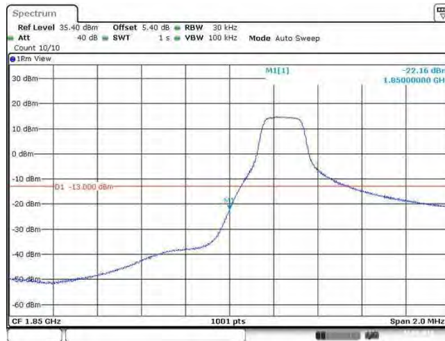
Band2_3MHz_64QAM_18615_15RB#0
