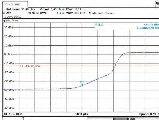
Band2_10MHz_64QAM_18650_50RB#0
