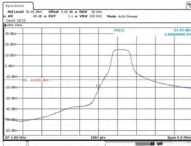
Band2_3MHz_QPSK_18615_15RB#0
