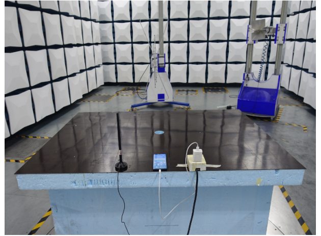
Radiated Disturbance Emissions (below 1GHz)
