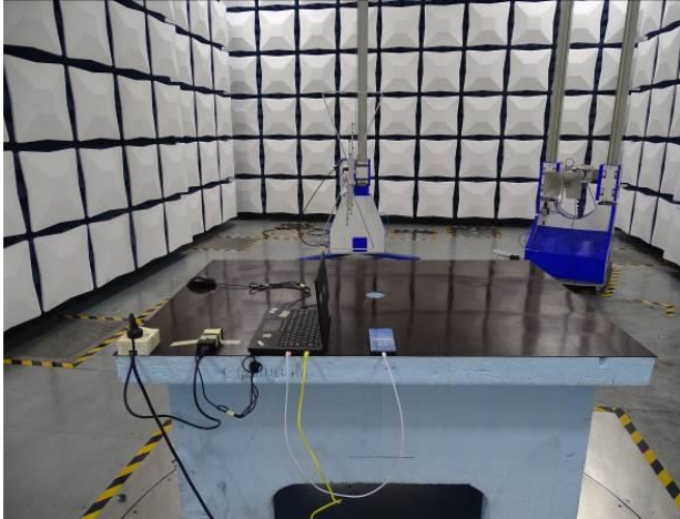
Radiated Disturbance Emissions (below 1GHz)
