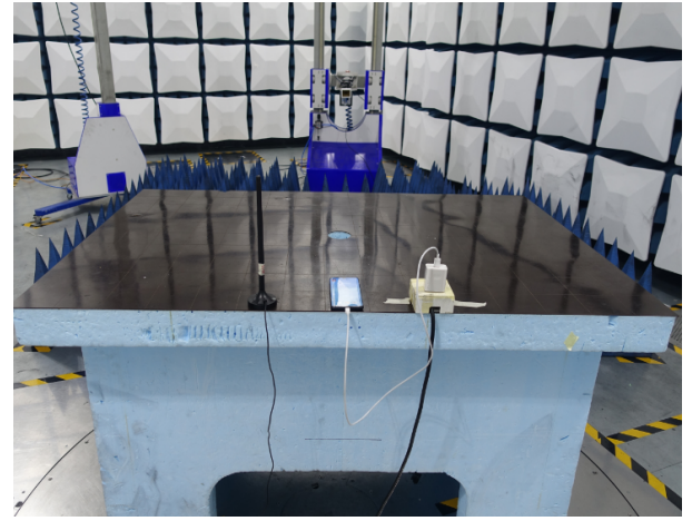
Radiated Disturbance Emissions (18GHz to 40GHz)
