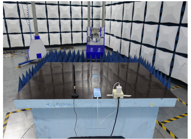
Radiated Disturbance Emissions (1GHz to 18GHz)
