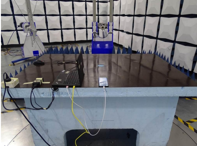
Radiated Disturbance Emissions (18GHz to 40GHz)
