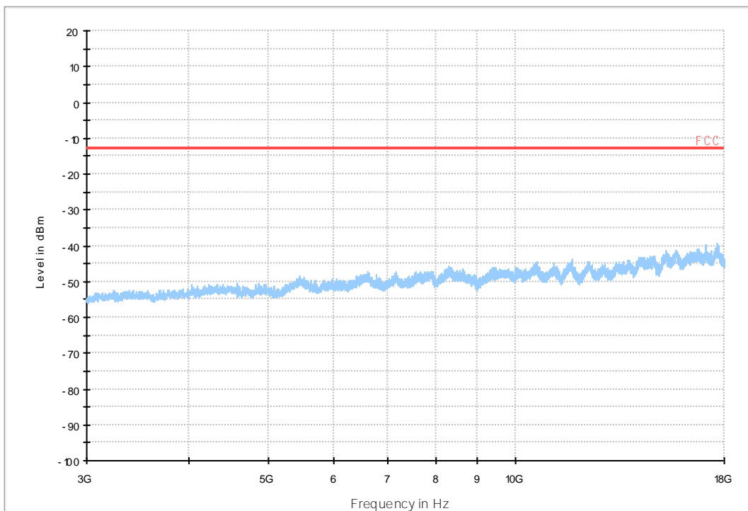
LT E FDD R SE-TX-DIRECT OR ABOVE 1.5G_H
