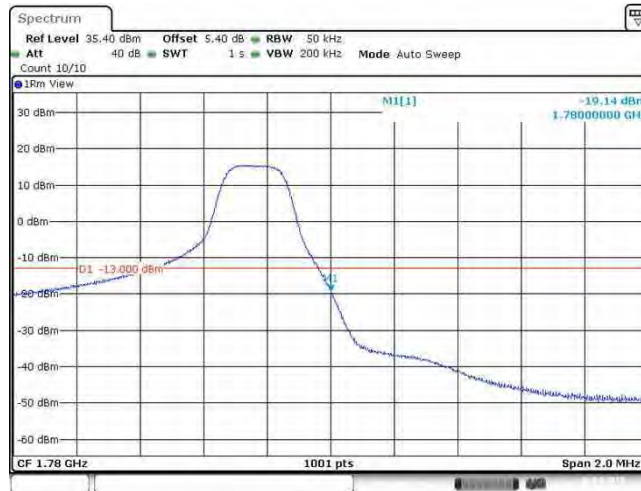
Band66_3MHz_16QAM_132657_15RB#0
