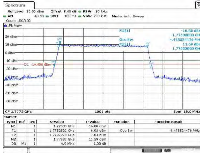
Band66_5MHz_64QAM_132647_25RB#0
