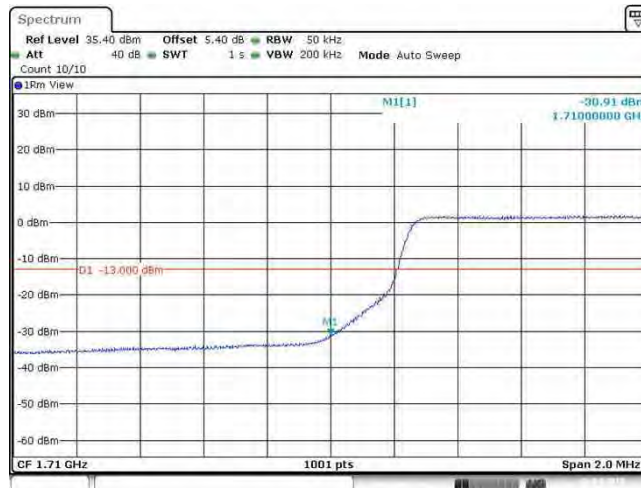
Band66_5MHz_QPSK_131997_25RB#0
