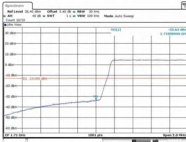
Band66_1.4MHz_64QAM_131979_6RB#0
