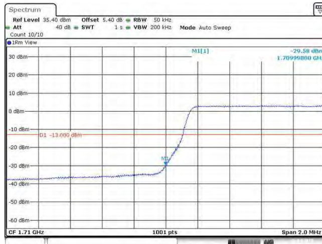
Band66_3MHz_64QAM_131987_15RB#0
