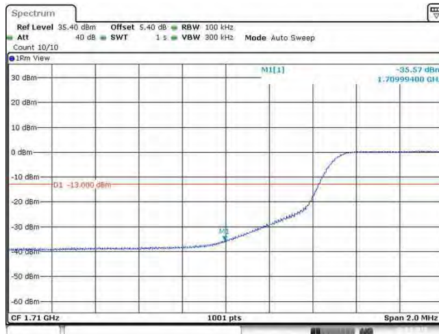
Band66_10MHz_16QAM_132022_50RB#0
