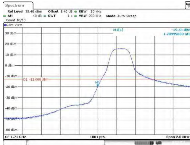
Band66_3MHz_64QAM_131987_15RB#0
