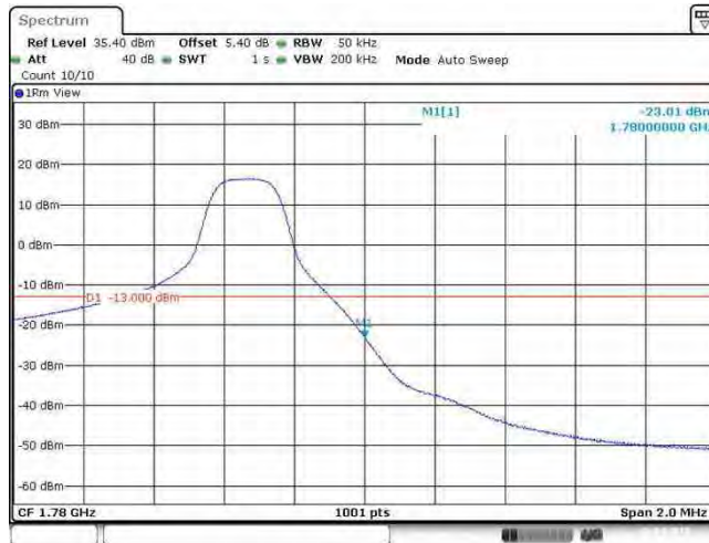
Band66_5MHz_QPSK_132647_25RB#0
