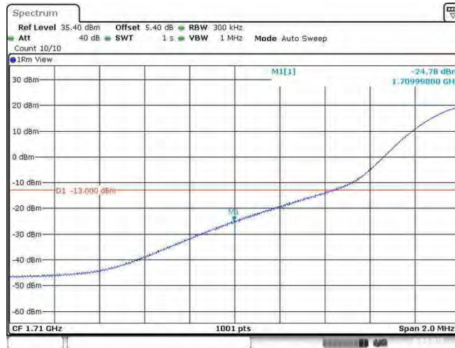
Band66_20MHz_64QAM_132072_100RB#0
