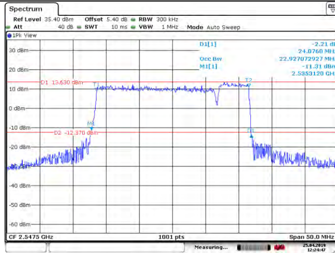
CA_41C_QPSK_100RB+25RB_40140+40257_PCC:100RB@0_SCC:25RB@0
