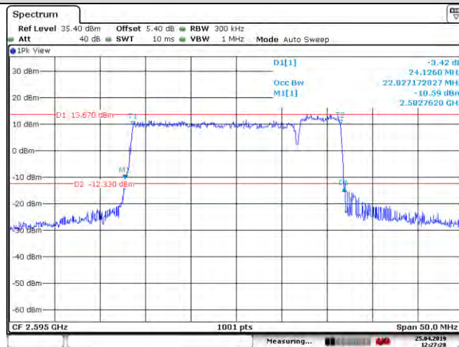
CA_41C_QPSK_100RB+25RB_40615+40732_PCC:100RB@0_SCC:25RB@0
