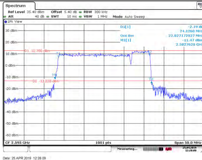
CA_41C_16QAM_100RB+25RB_41090+41207_PCC:100RB@0_SCC:25RB@0
