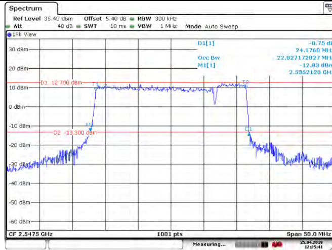
CA_41C_16QAM_100RB+25RB_40615+40732_PCC:100RB@0_SCC:25RB@0
