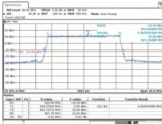
Band26_5MHz_64QAM_26765_25RB#
