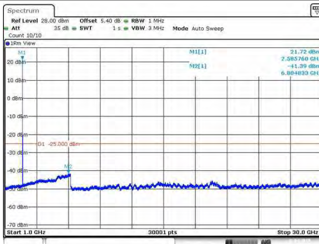
Band41_20MHz_16QAM_40640_1RB#0
