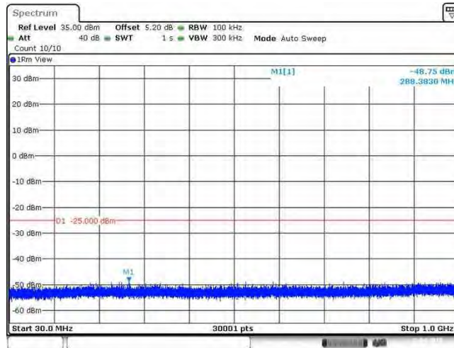
Band41_20MHz_64QAM_40140_1RB#0
