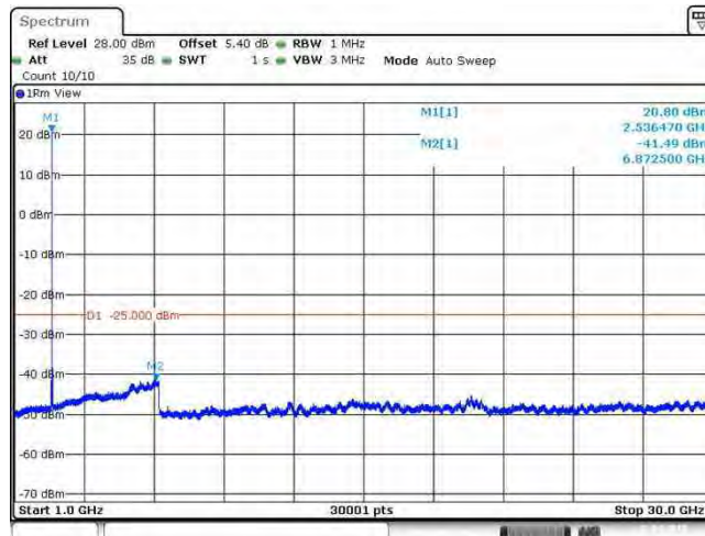
Band41_20MHz_64QAM_40140_1RB#0
