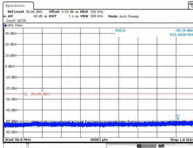
Band41_20MHz_16QAM_40140_1RB#0
