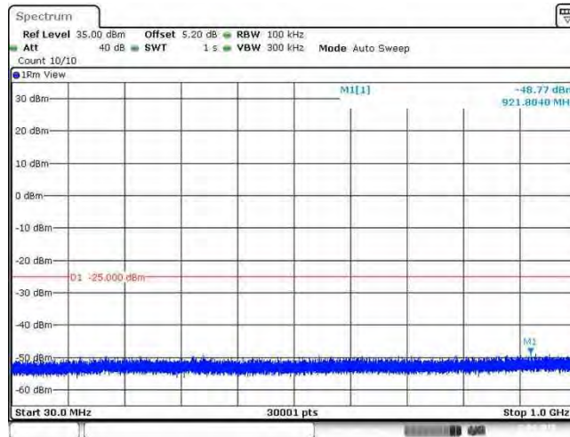
Band41_20MHz_64QAM_40640_1RB#0
