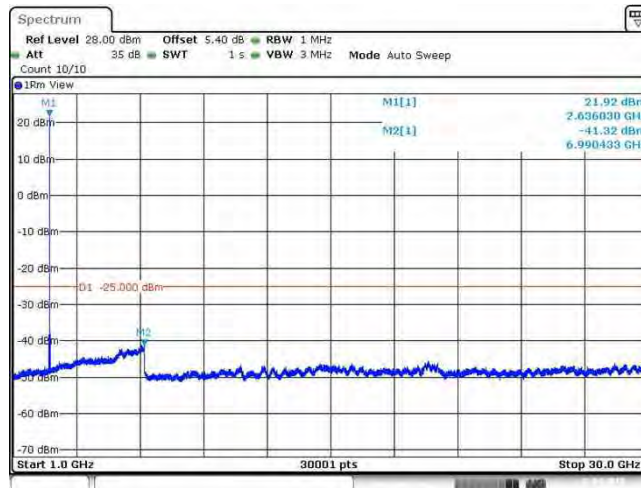
Band41_20MHz_QPSK_41140_1RB#0
