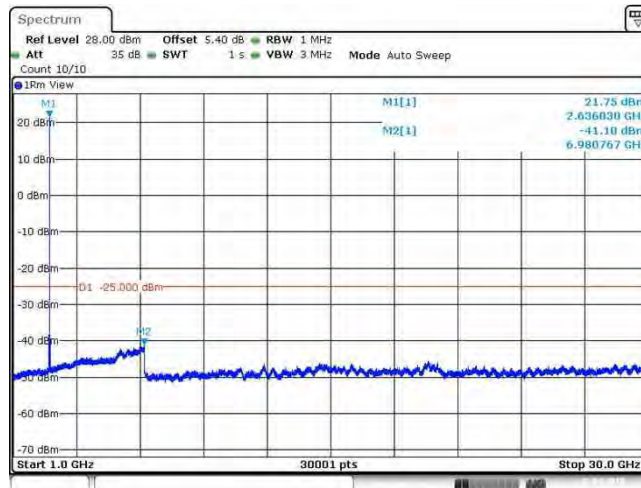
Band41_20MHz_64QAM_41140_1RB#0
