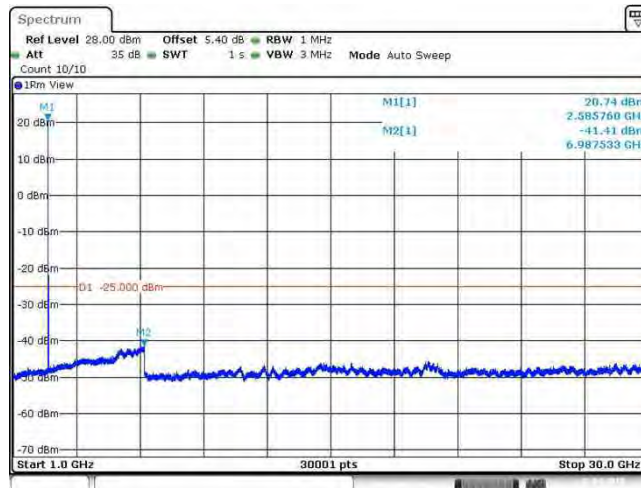
Band41_20MHz_64QAM_40640_1RB#0
