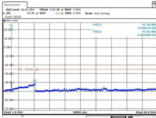
Band41_20MHz_16QAM_40140_1RB#0
