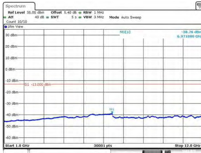
Band12_10MHz_64QAM_23095_1RB#0
