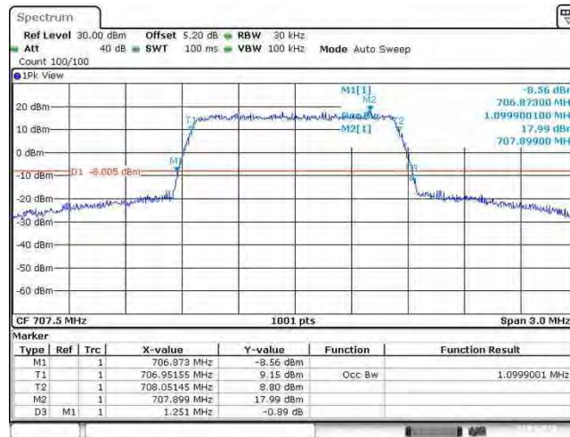
Band12_1.4MHz_16QAM_23095_6RB#0
