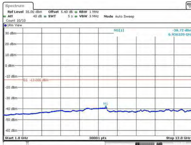
Band12_10MHz_64QAM_23130_1RB#0
