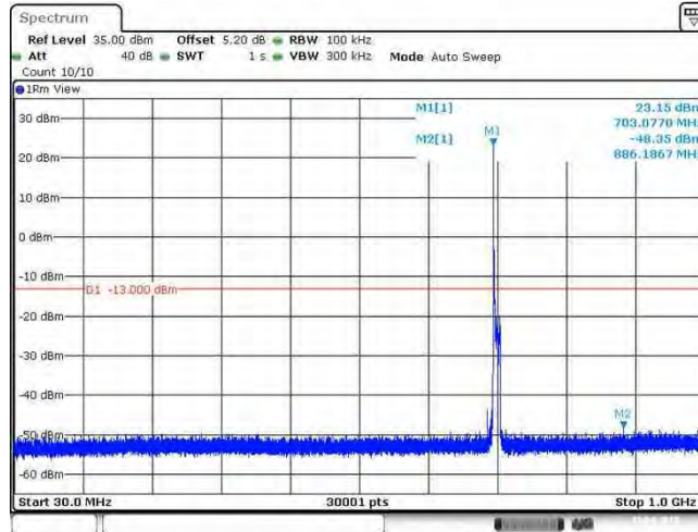
Band12_10MHz_QPSK_23095_1RB#0
