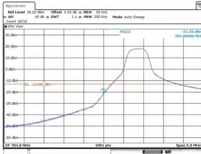
Band17_5MHz_64QAM_23755_25RB#0
