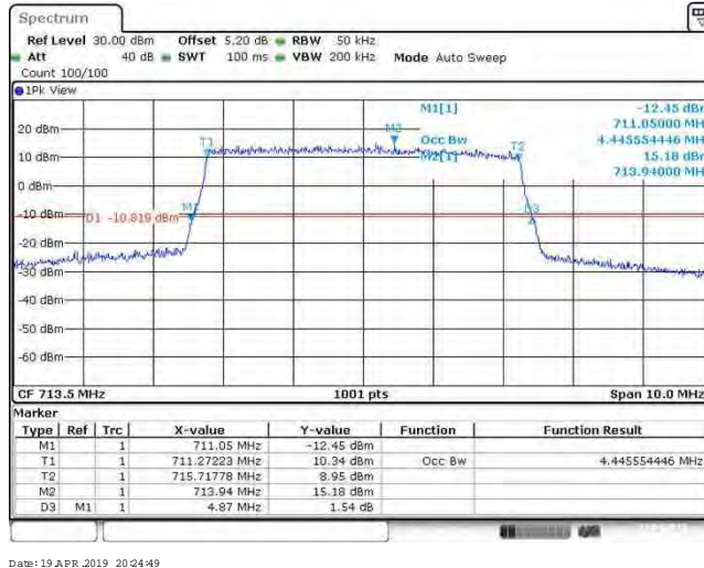
Band17_5MHz_16QAM_23755_25RB#
