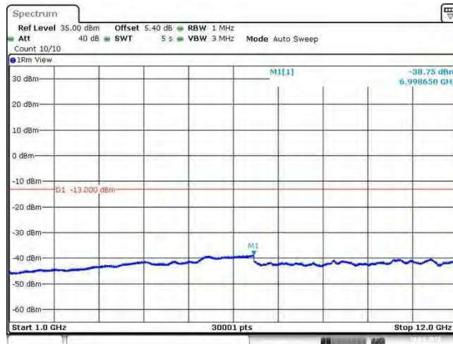
Band17_10MHz_64QAM_23800_1RB#0
