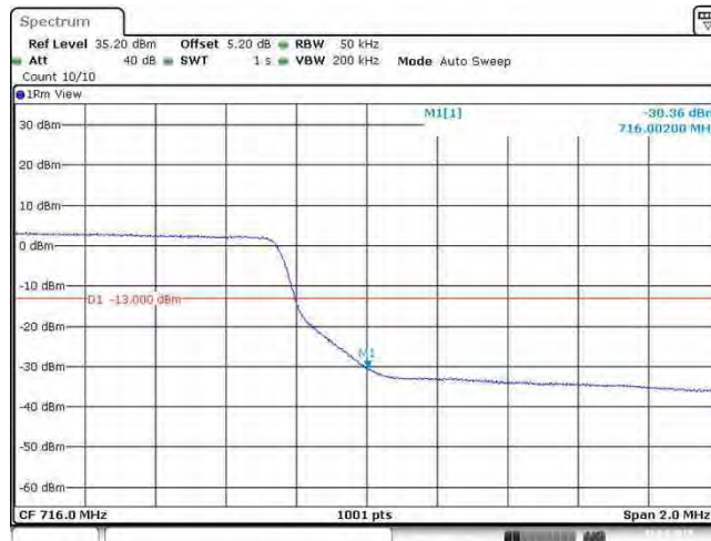
Band17_5MHz_QPSK_23825_25RB#0
