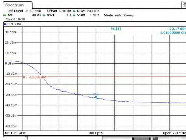
Band2_15MHz_64QAM_19125_75RB#0
