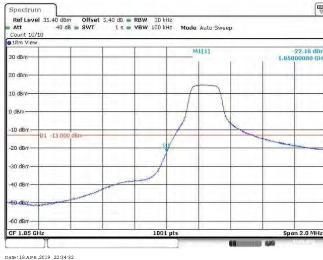
Band2_3MHz_64QAM_18615_15RB#0
