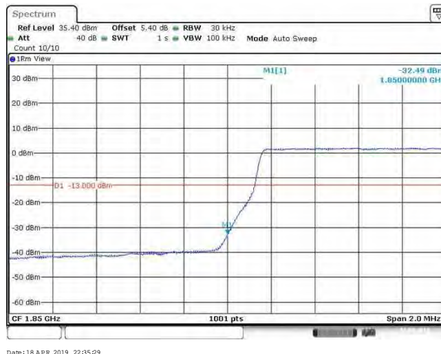
Band2_3MHz_64QAM_19185_1RB#14
