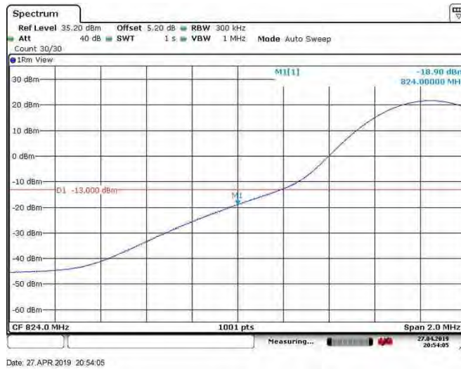
Band26_15MHz_64QAM_26865_75RB#0
