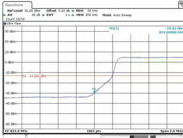
Band26_5MHz_QPSK_26815_25RB#0
