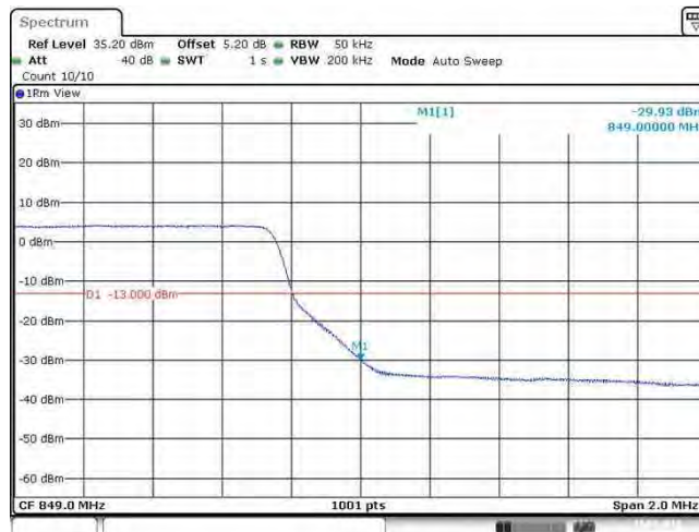
Band26_5MHz_QPSK_27015_25RB#0
