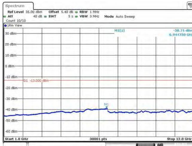
Band26_15MHz_QPSK_26965_1RB#0
