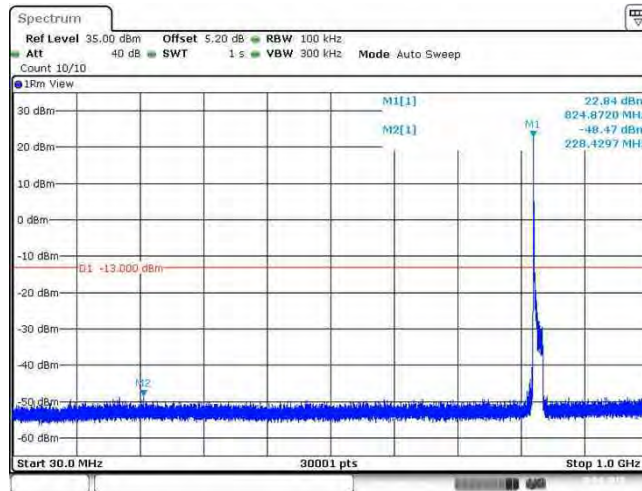
Band26_15MHz_16QAM_26865_1RB#0
