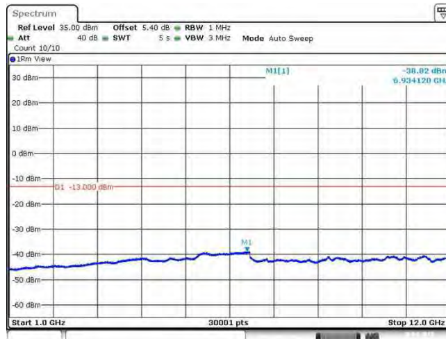
Band26_15MHz_16QAM_26915_1RB#0
