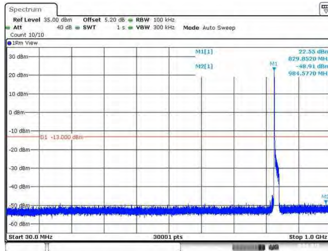
Band26_15MHz_64QAM_26915_1RB#0
