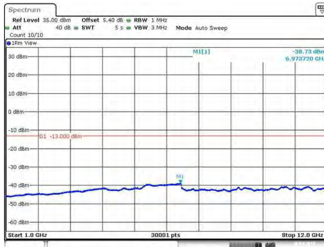
Band26_15MHz_64QAM_26865_1RB#0
