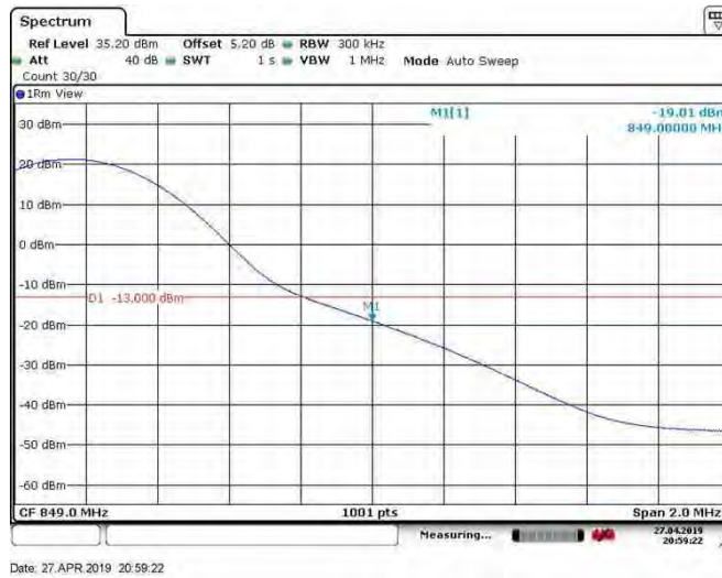
Band26_15MHz_64QAM_26965_75RB#0
