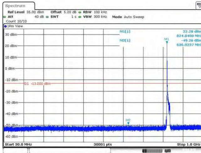
Band26_15MHz_64QAM_26865_1RB#0
