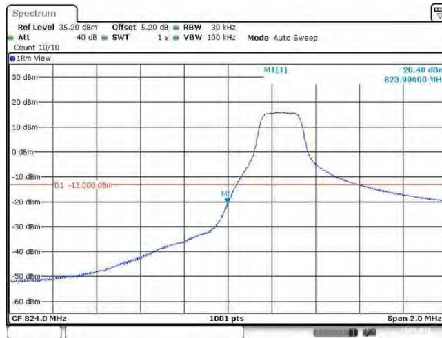
Band26_3MHz_16QAM_26805_15RB#0
