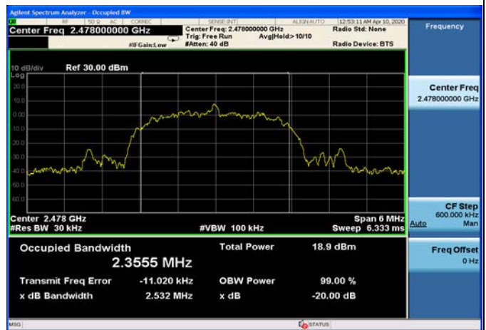
BT UHD 2M 8DPSK CH37, Carrier frequency (MHz): 2478
