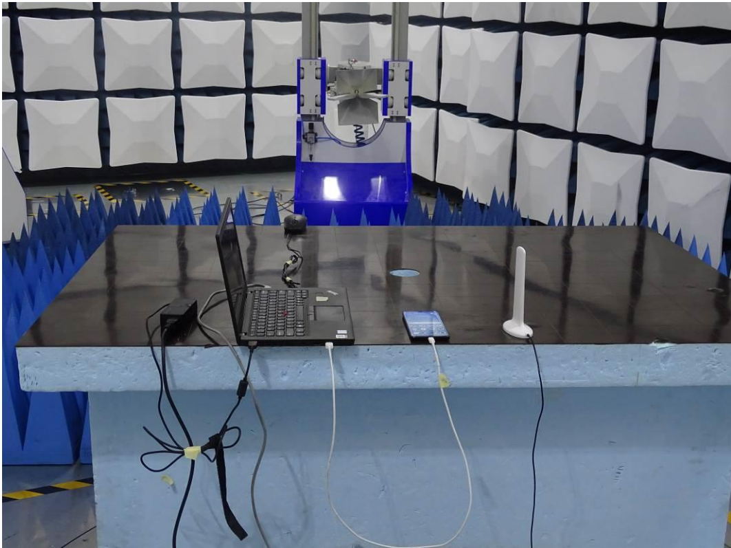
Radiated Disturbance Emissions (1GHz to18GHz)
