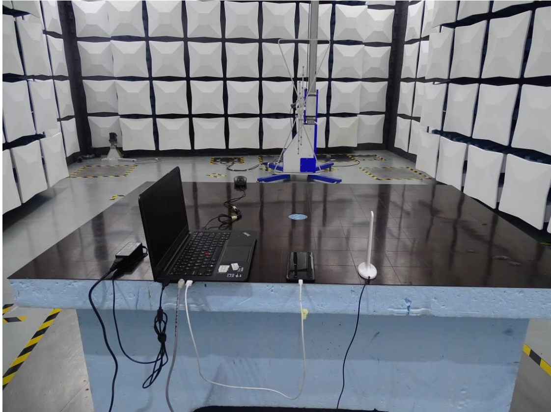
Radiated Disturbance Emissions (below 1GHz)
