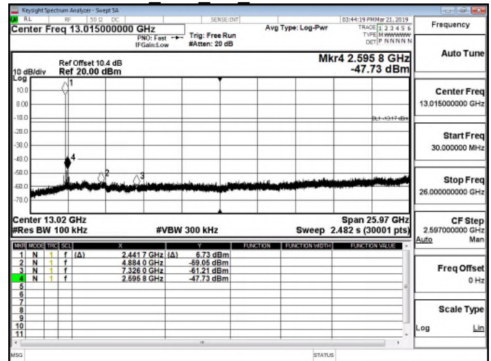
FCC_15_247_BT4\Spurious Emission_BLE_1M_MidCH20-2442
