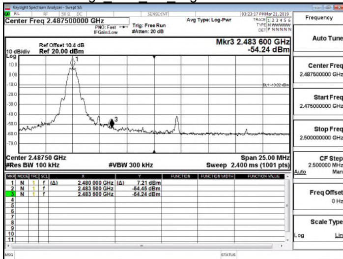
FCC_15_247_BT4\Band Edge_BLE_1M_HighCH39-2480
