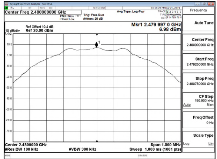
FCC_15_247_BT4\Reference Level_BLE_1M_HighCH39-2480
