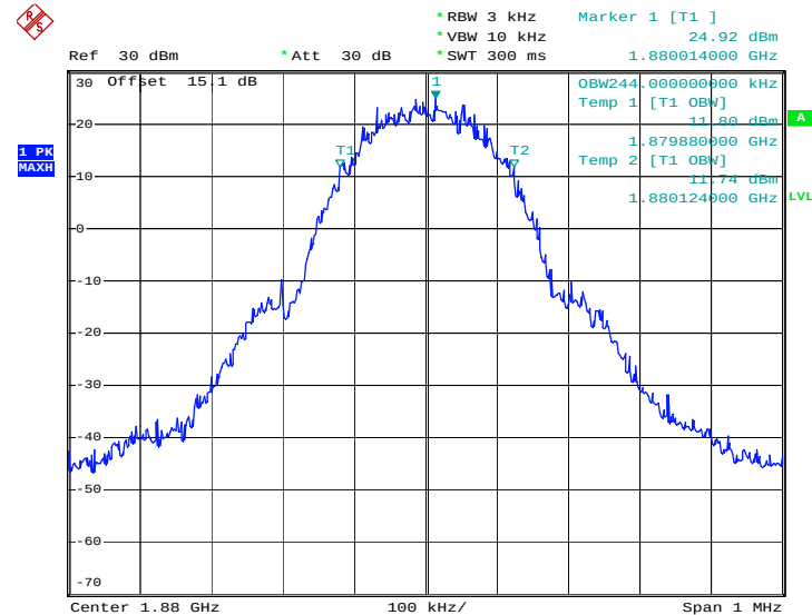
99% Occupied Bandwidth Plot on Channel 661
