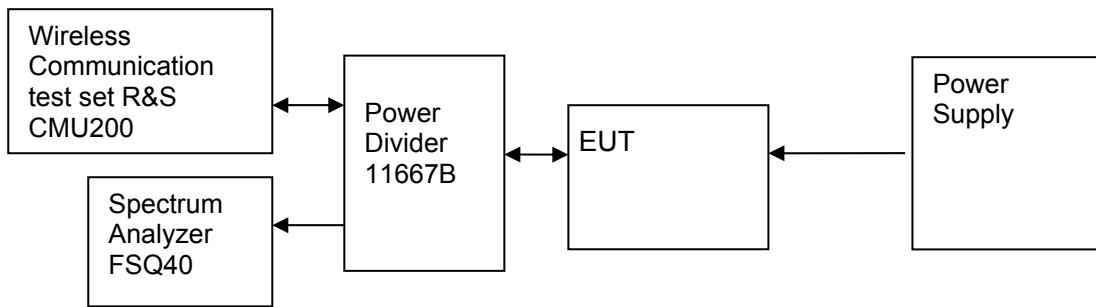
Figure 1. Test Set-up
