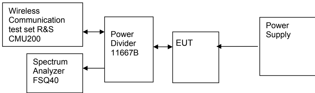
Figure 2. Test Set-up
