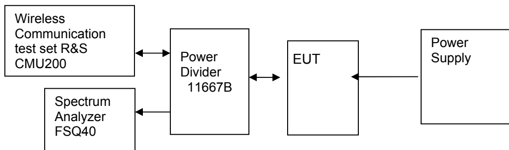
Figure 3. Test Set-up
