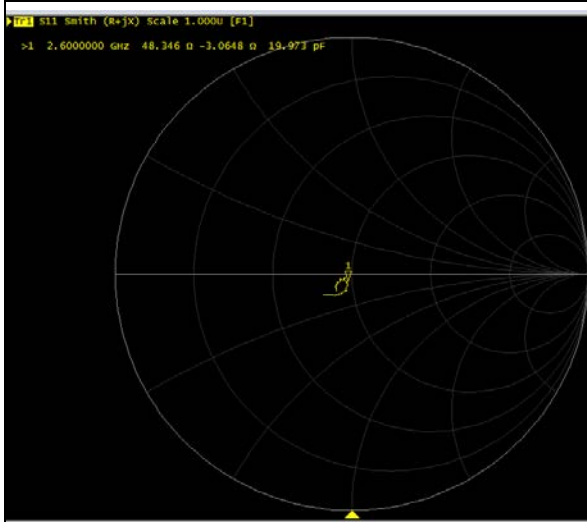
Impedance Test-Body
