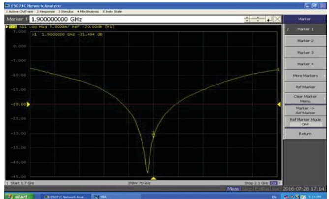
Return Loss-Body
