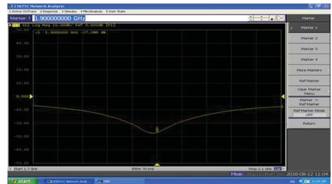
Return Loss-Body
