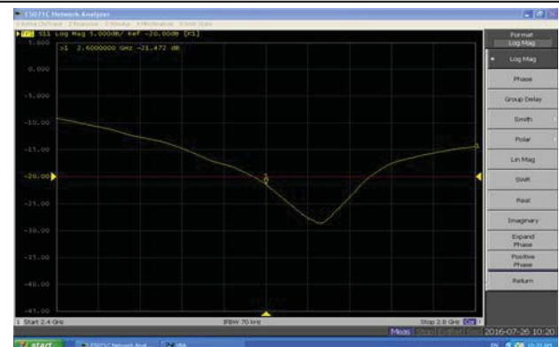
Return Loss-Body
