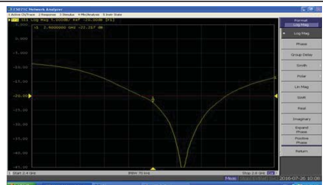
Return Loss-Body
