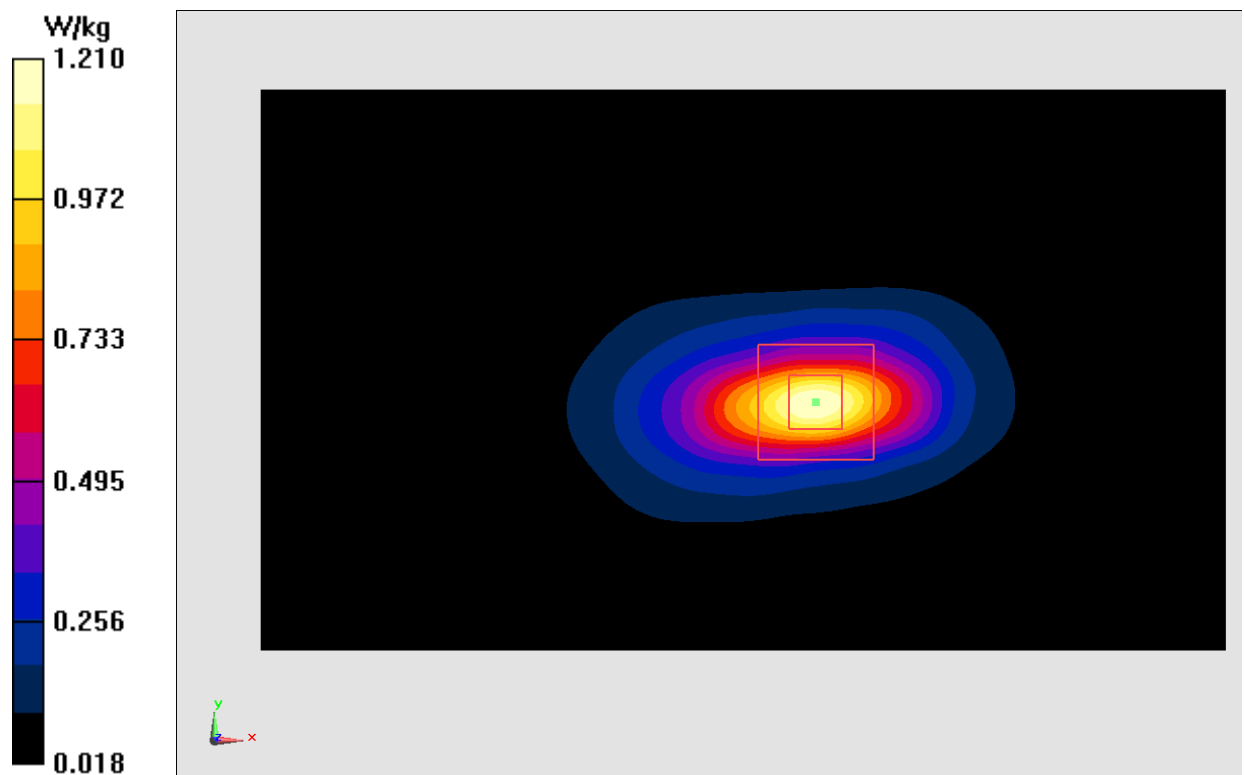
Fig.4 1900 MHz
