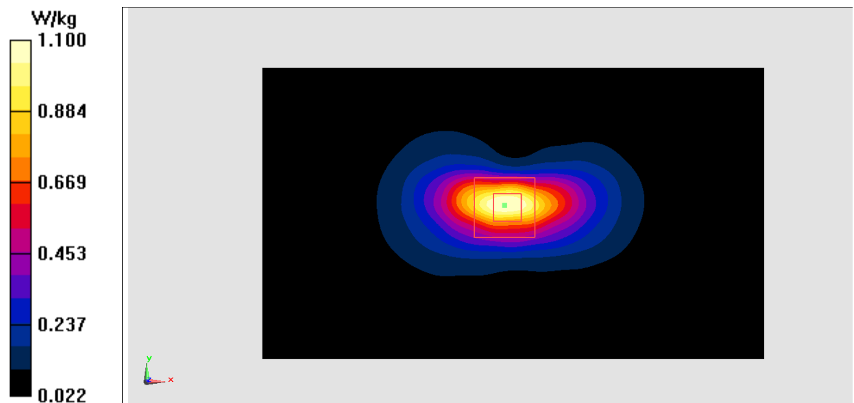
Fig.8 1700 MHz
