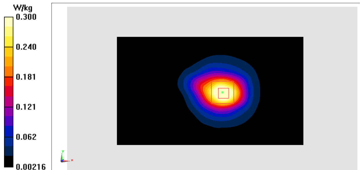
Fig.20 2450 MHz
