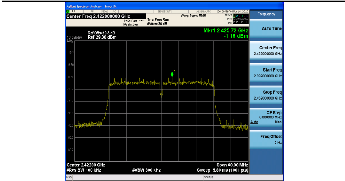
11N40SISO_Ant1_2422_0.009~30
