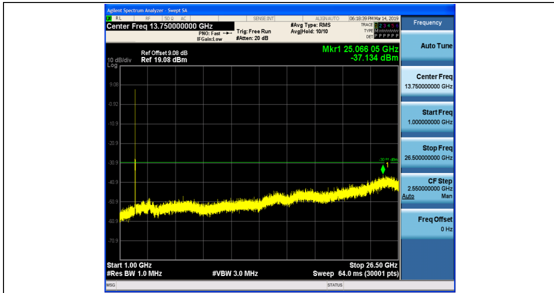
11N20SISO_Ant1_2417_0~Reference
