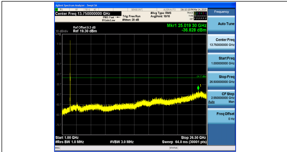
11G_Ant1_2457_0~Reference
