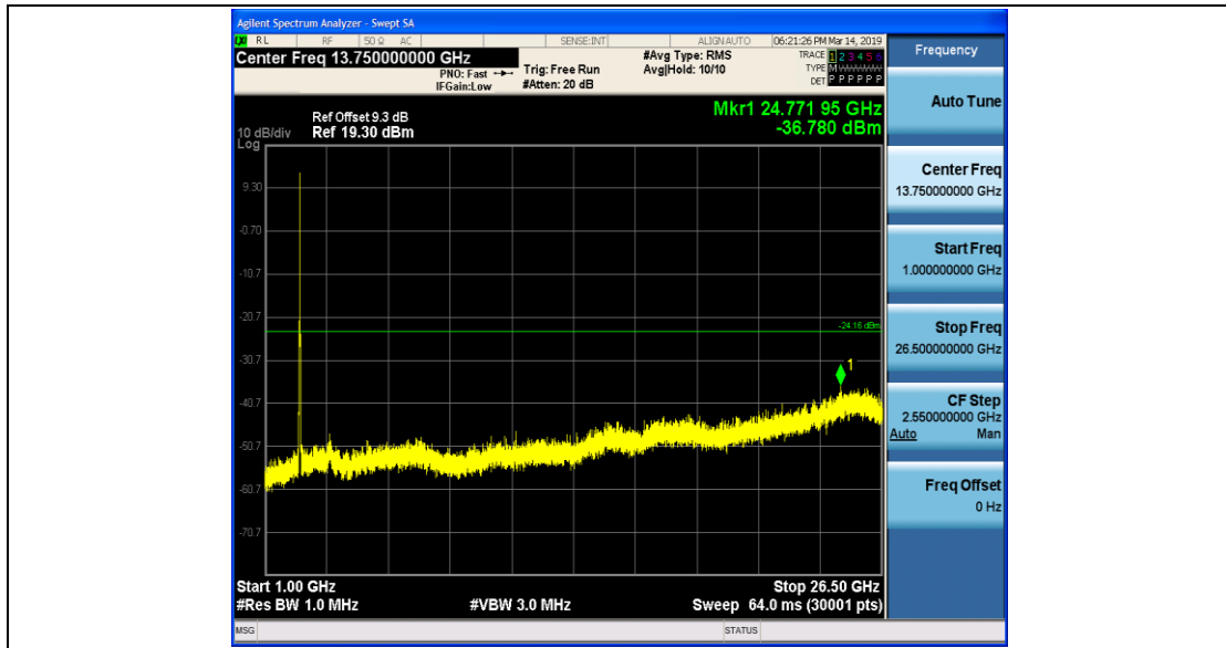
11N20SISO_Ant1_2457_0~Reference
