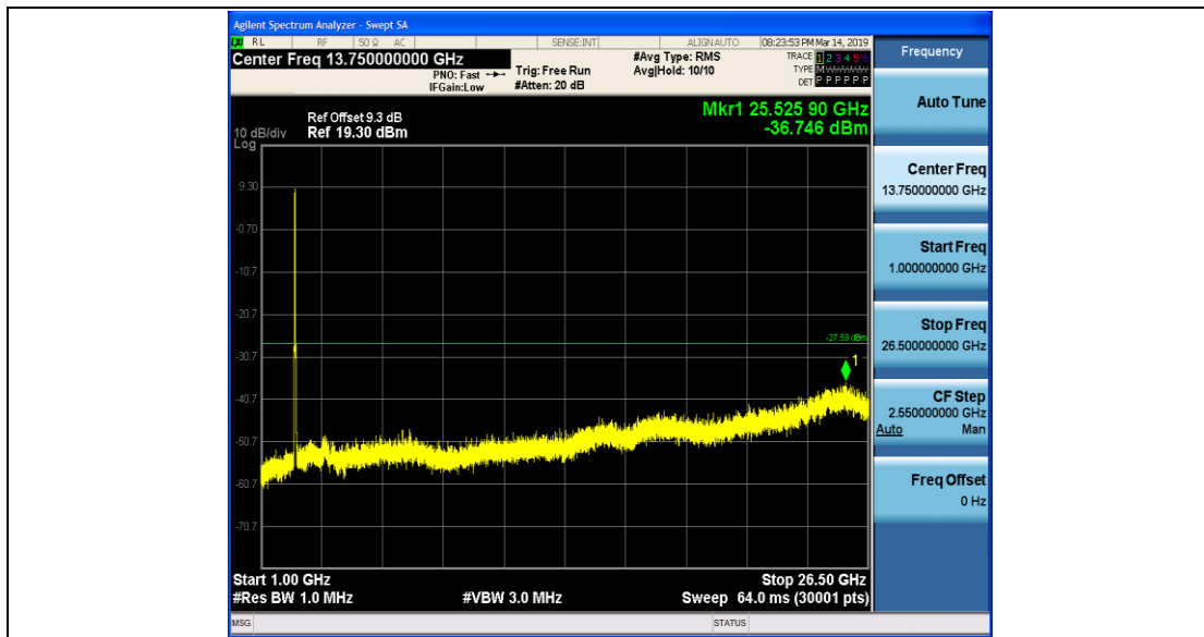
11N40SISO_Ant1_2437_0~Reference
